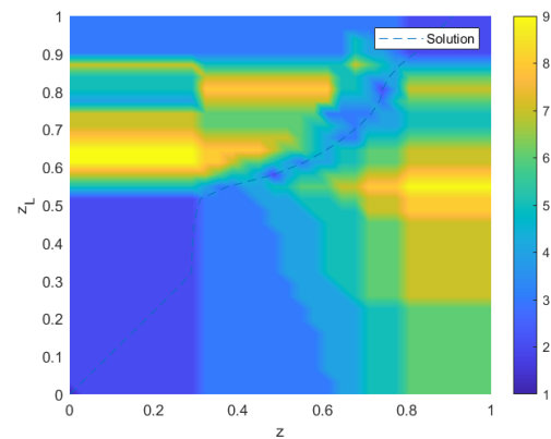
(b) Convergence map for TR algorithm
