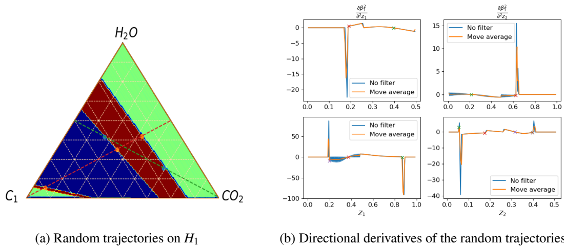
Figure 5: Full and directional evaluations of second order behavior for ternary compositional kernel.
