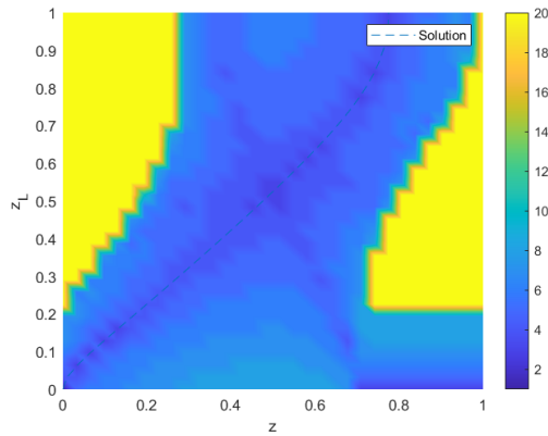
(a) Convergence map for pure newton
