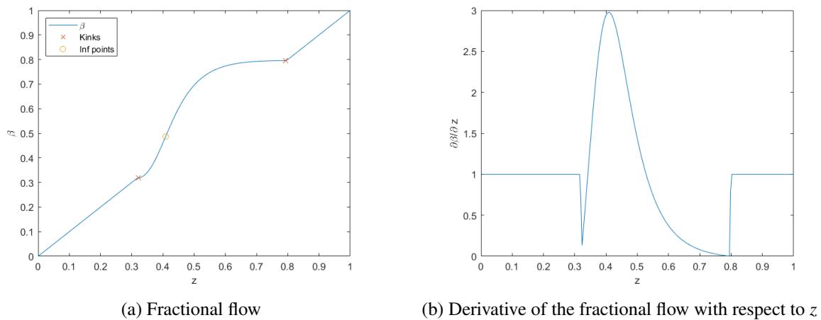
Figure 2: Binary incompressible compositional kernel
