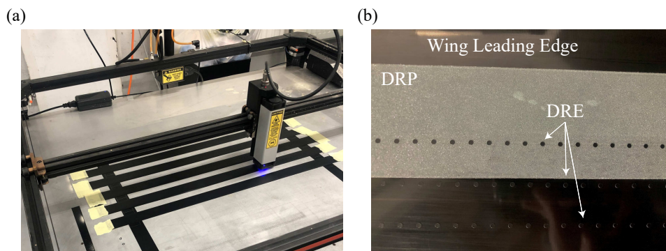
FIGURE 2.4: (a) Production of multiple DRE arrays by laser cutting black PVC foil using the Toolie machine. (b) Detail of the wing leading edge with spray adhesive DRP and DRE array applied.
