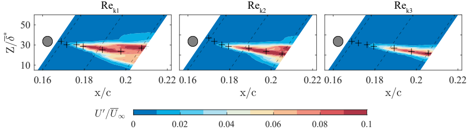
FIGURE 4.6: U' contours at constant wall-normal distance y/\delta^* = 1.7 for Re_{k1} = 251 , Re_{k2} = 222 , Re_{k3} = 198 . Highest U' locii (+) computed at the same chord location of the acquired yz planes; IDRE top view (grey circle).
