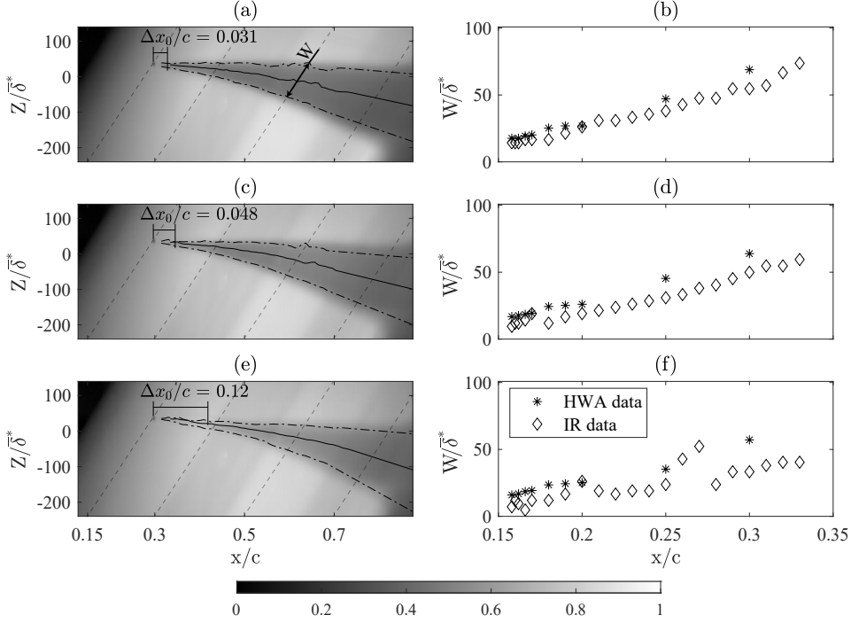
FIGURE 4.2: (a, c, e) IR thermography fields and (b, d, f) estimation of wedge width ( W ) evolution along wing chord for x_{IDRE}/c=0.15 and (a-b) Re_{k1} , (c-d) Re_{k2} , (e-f) Re_{k3} . (a, c, e) Flow comes from the left, wedge middle point (- line); linear interpolation of the wedge limits (-. lines); wedge origin distance from the element ( \Delta x_0/c ). (b, d, f) Values collected from post-processing of HWA (*) and IR ( \diamond ) data.
