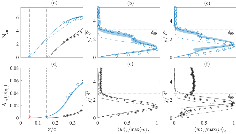
FIGURE 3.10: PIV and NPSE \lambda_1 mode (a) N_{\text{eff}} and (d) A_{\text{int}} for Re_k=18 (*) and Re_k=24 (o) with x_{\text{DRE}}/c (-), A_0 (x). (b-e) Shape functions of the \lambda_1 and (c-f) \lambda_2 mode at x/c=0.30 for the NPSE (full line), LPSE (- -) and FFT shape functions from PIV (symbols). Experimental \delta_{99} (- -), NPSE matching sensitivity (shadowed areas).
