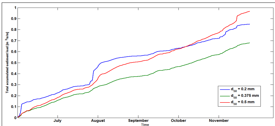
FIGURE 5.41 COMPARISON OF TOTAL ACCUMULATED LOAD FOR DIFFERENT SEDIMENT GRAIN SIZE
