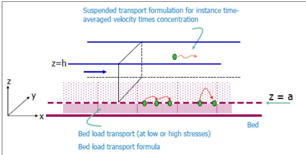
FIGURE 2.4 SEDIMENT TRANSPORT MODES (SOURCE: BOSBOOM J & STIVE M, 2012)
