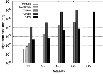
Fig. 9. The algorithm run time of PageRank on 5 datasets with different graph processing systems (the vertical axis has a logarithmic scale, missing bars are explained in the text).
