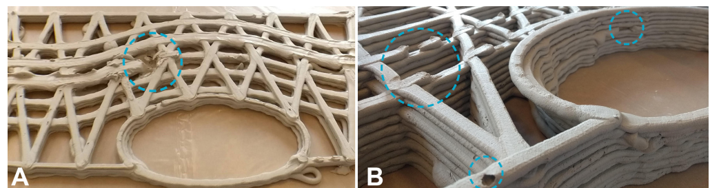
Figure 19. Damages and discontinuities caused by Air Shots. (A) A damage affected multiple layers (marked in cyan). (B) Discontinuity within layers (marked in cyan).
