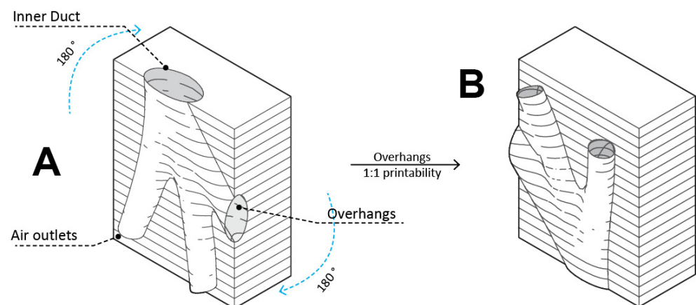
Figure 9. The outlets, overhangs, and inner ducts, seen within the part chosen for prototyping. (A) The original orientation of the part. (B) The part rotated 180^\circ for prototyping (the blue arrows indicate the rotation).
