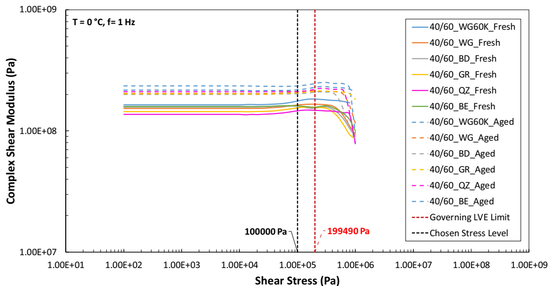
Fig. A2. Mastics amplitude sweep test results. T = 0\text{ }^{\circ}\text{C} , f = 1\text{ Hz} .
