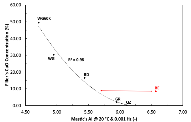
Fig. 7. Relationship between fillers' CaO concentration and mastics' complex shear modulus ageing indices at 0.001 Hz and 20 °C.
