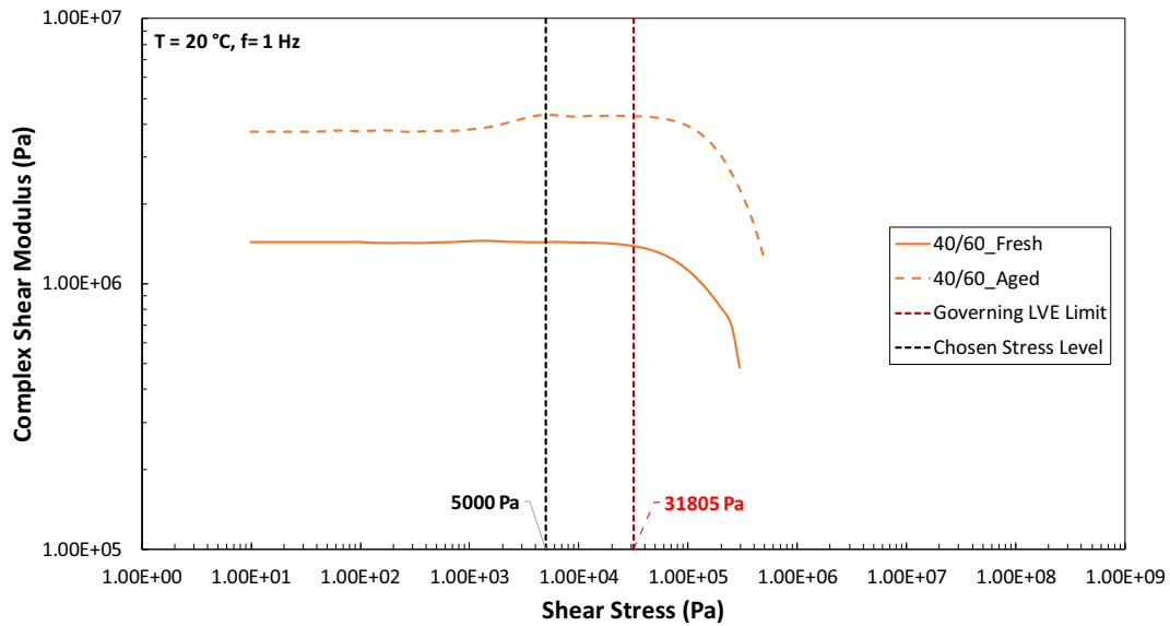
Fig. A10. Bitumen amplitude sweep test results. T = 20 °C, f = 1 Hz.
