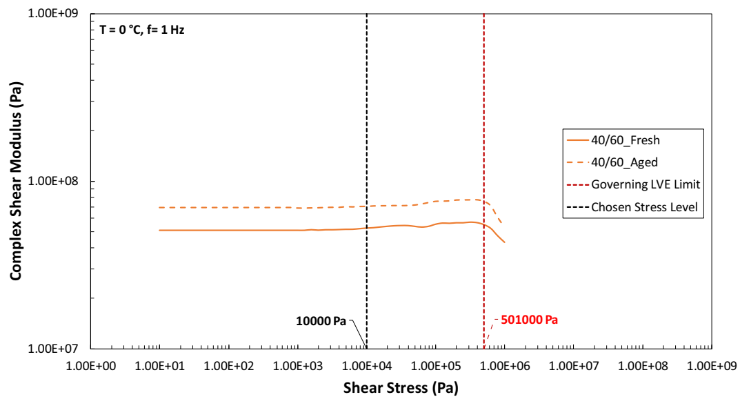
Fig. A8. Bitumen amplitude sweep test results. T = 0\text{ }^{\circ}\text{C} , f = 1\text{ Hz} .
