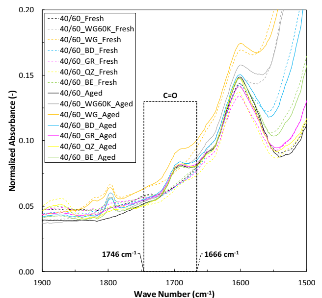
Fig. 8. Fresh and aged bitumen and mastics infrared spectra, carbonyls close-up.
