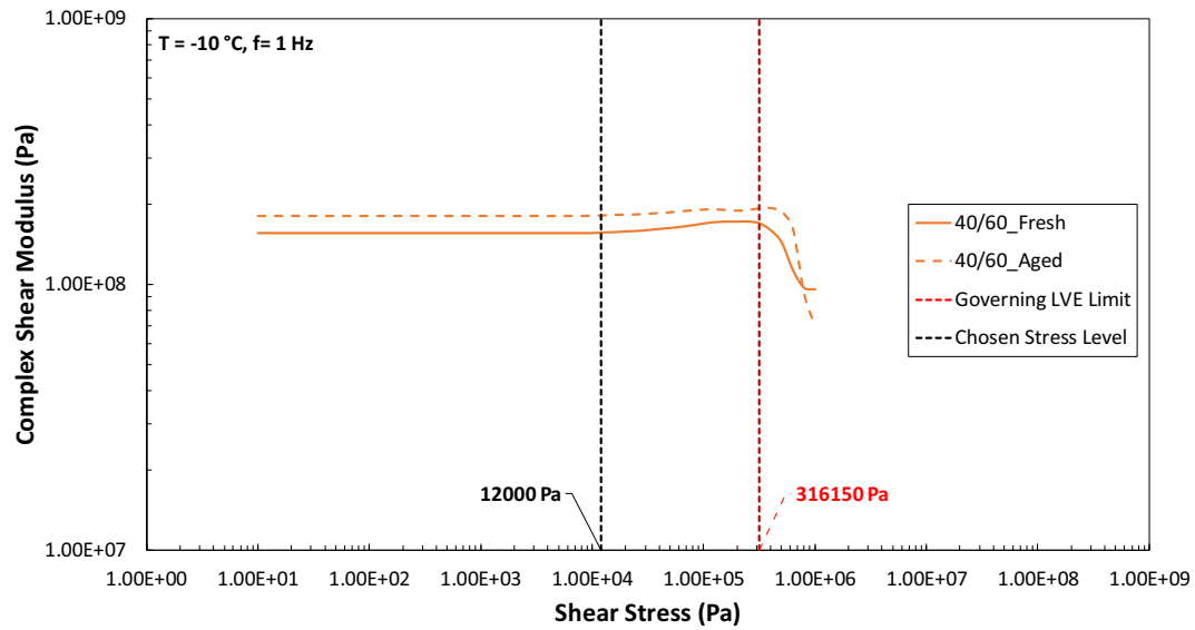
Fig. A7. Bitumen amplitude sweep test results. T = -10\text{ }^{\circ}\text{C} , f = 1\text{ Hz} .
