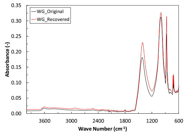
Fig. 14. Original and recovered filler WG infrared spectra.
