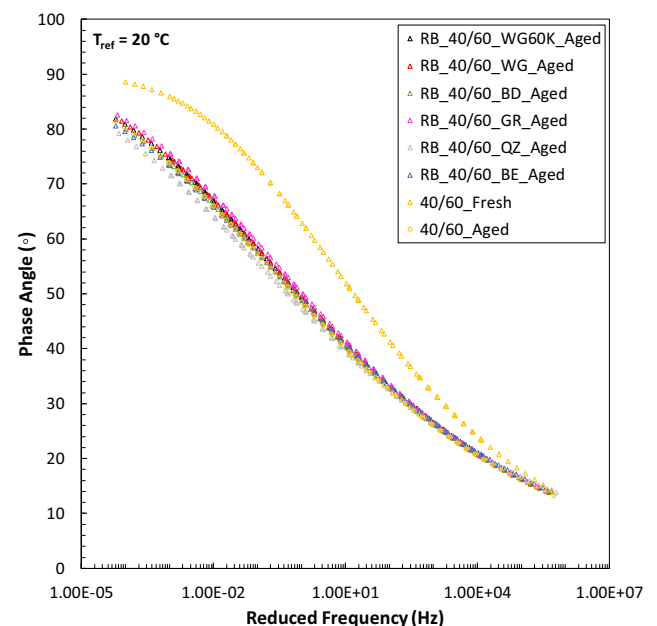
Fig. 11. Fresh, aged and recovered bitumen phase angle master-curves.
