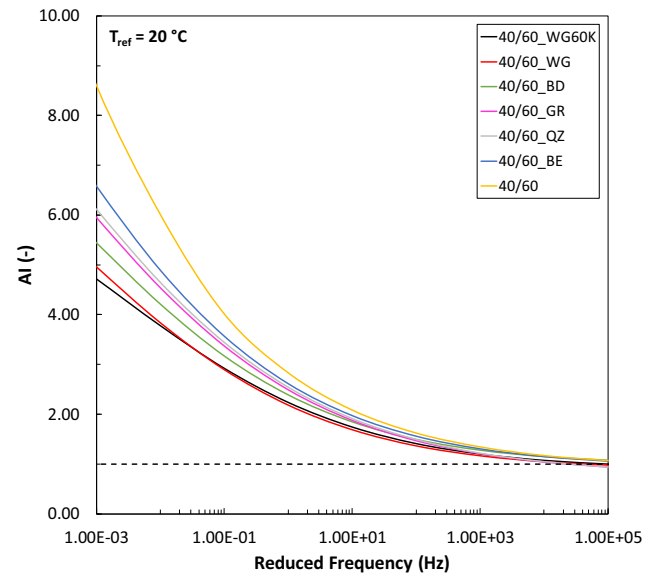
Fig. 5. Complex shear modulus ageing indices as a function of the reduced frequency at 20 °C.
