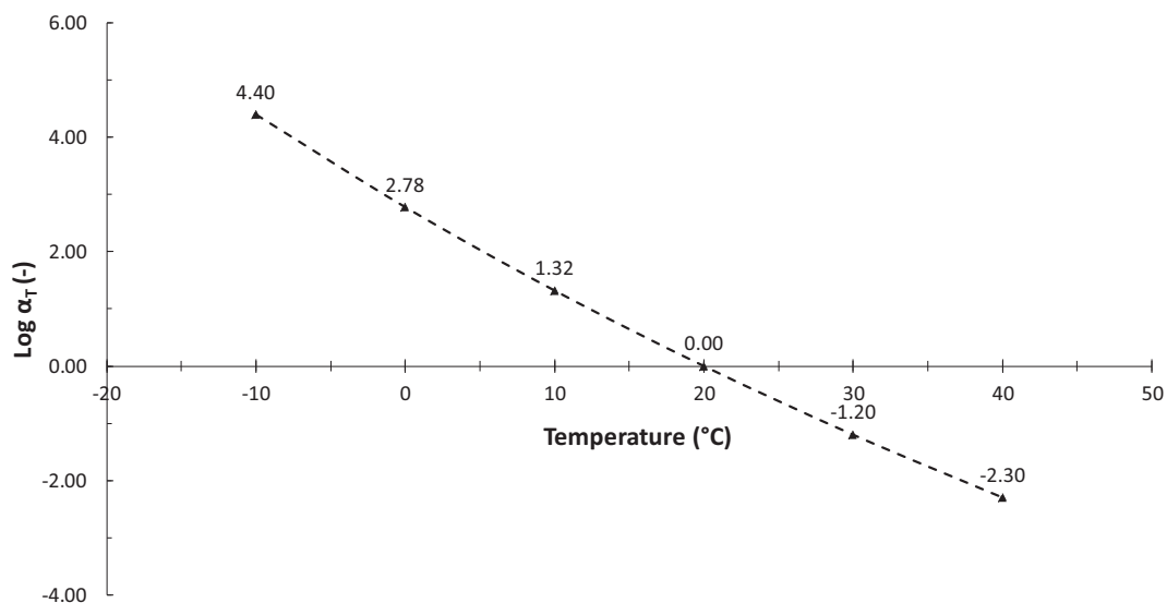
Fig. B13. WLF shift factors. 40/60_Fresh.
