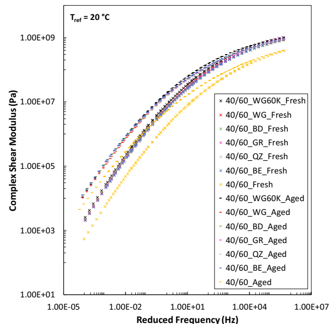
Fig. 3. Bitumen and mastics complex shear modulus master-curves at fresh and aged state.
