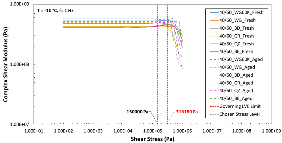
Fig. A1. Mastics amplitude sweep test results. T = -10\text{ }^{\circ}\text{C} , f = 1\text{ Hz} .
