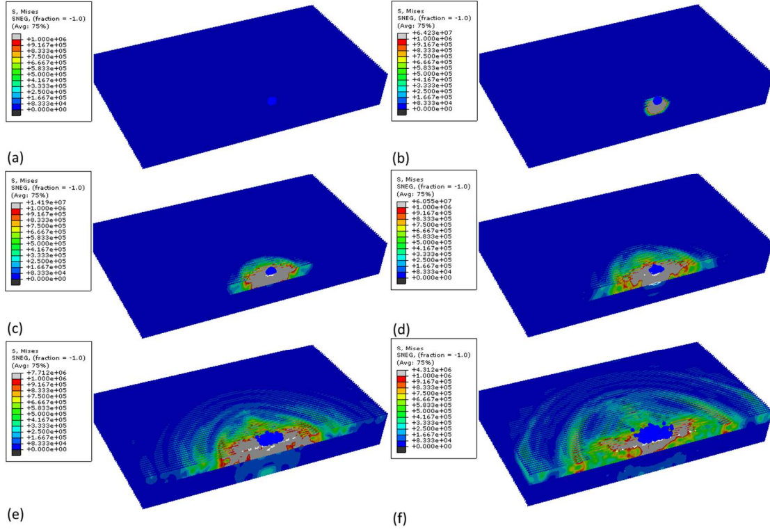
Figure 9 Simulation of a single raindrop impact. (a-f) cross-sectional views of von Mises stress contours at six time instants (0 \mu s, 1 \mu s, 5 \mu s, 10 \mu s, 20 \mu s, 30 \mu s) using the raindrop diameter of 2 mm and the impact speed of 90 \text{ms}^{-1} .
