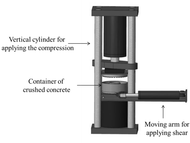
Figure 5-3: The schematic of the Shear-Compression Machine (SCM).
