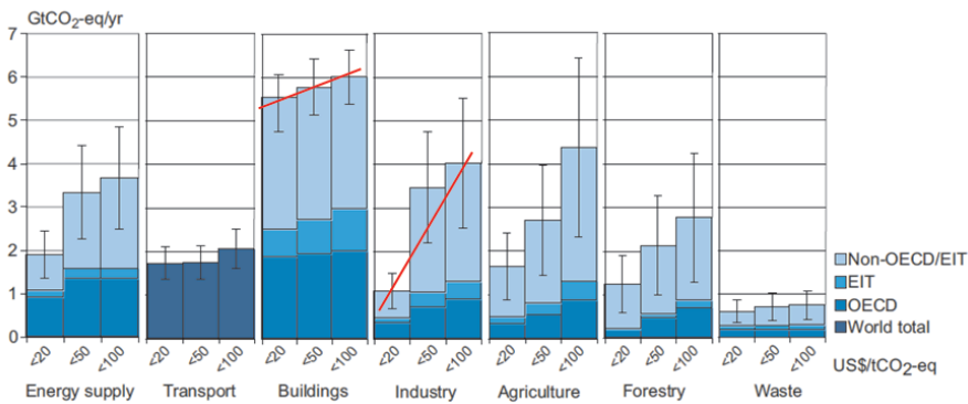
Figure 1-7: Estimated sectoral economic potential for global mitigation for different regions and different cost levels (20$, 50$ and 100$ per ton of avoided CO 2 )[14].
