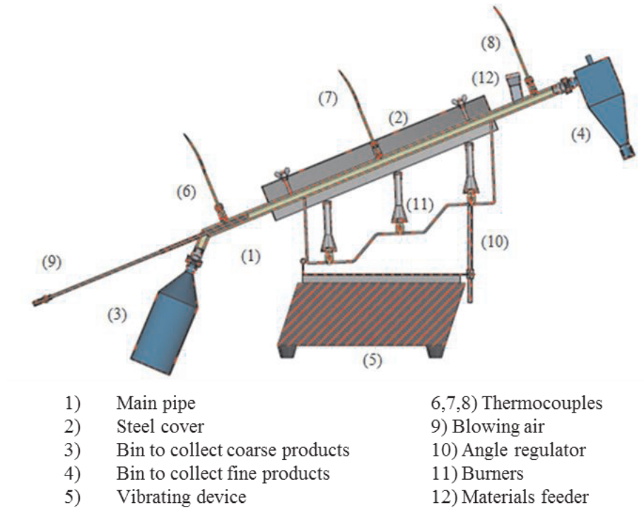
Figure 7-4: HAS set-up to heat AF and separate finer fraction (0-0.250mm) from coarser fraction (0.250-4mm).
