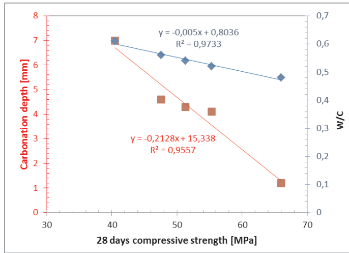
Figure 5-17: correlation between compressive strength and carbonation depth and compressive strength and w/c ratio of RAC samples.
