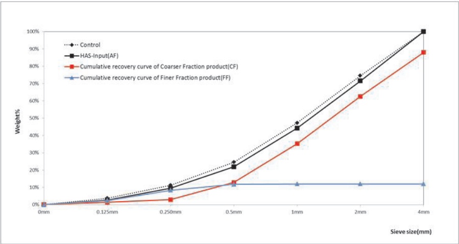
Figure 7-8: Reconstructed cumulative curve of the input materials (control curve) in comparison with the actual cumulative curve of HAS-Input.
