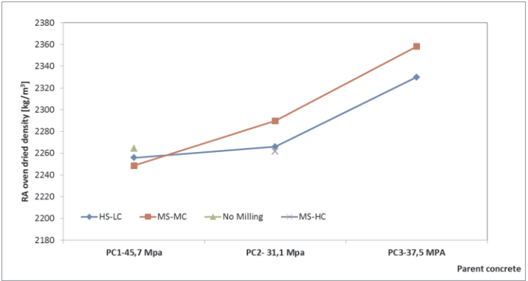
Figure 5-10: The effect of the PC type and milling intensity on oven dried density of RA.
