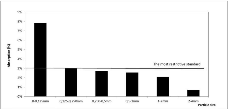
Figure 7-18: Estimated water absorption of all fractions obtained from a recycling process at 500°C with 300 seconds milling.
