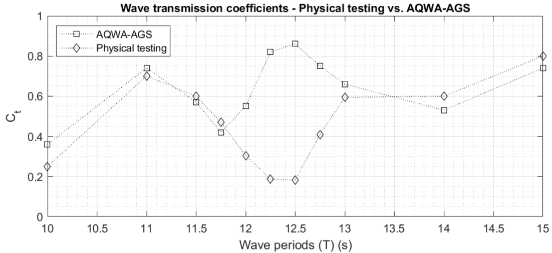
Fig. 9. Evaluation of numerical and physical tested transmission coefficients values.
