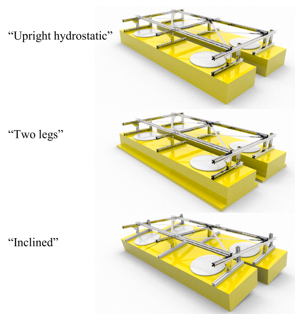
Fig. 2. Sectional model configurations.
