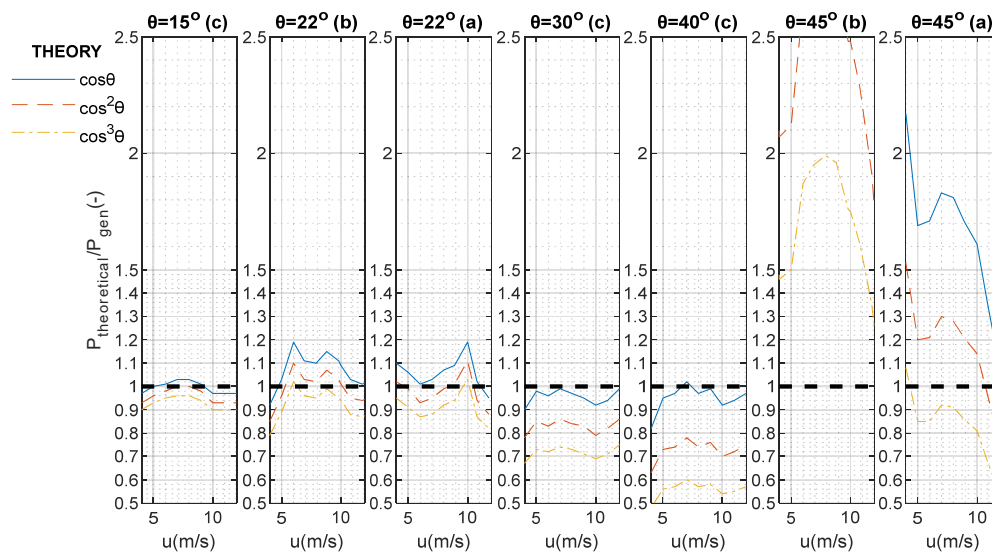
Figure 9. Ratio of theoretical power estimation from 3 different yaw misalignment theories at different skew angles ( 15^\circ , 22^\circ , 30^\circ , 40^\circ , 45^\circ ) with the experimentally derived generated power at these skew angles for (a) 5-bladed upwind, (b) 3-bladed downwind, and (c) 3-bladed downwind configurations.
