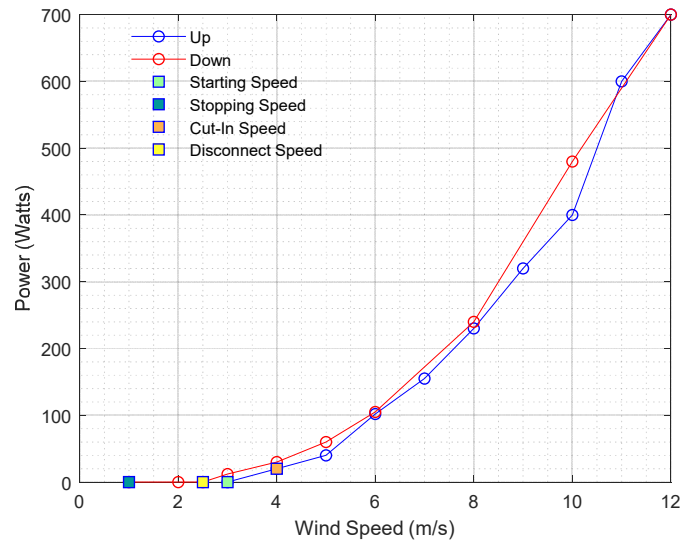
Figure 21. Power curve recordings with an increasing (up) wind speed and then decreasing (down) wind speed. Characterizing wind speeds are noted in the legend box.
