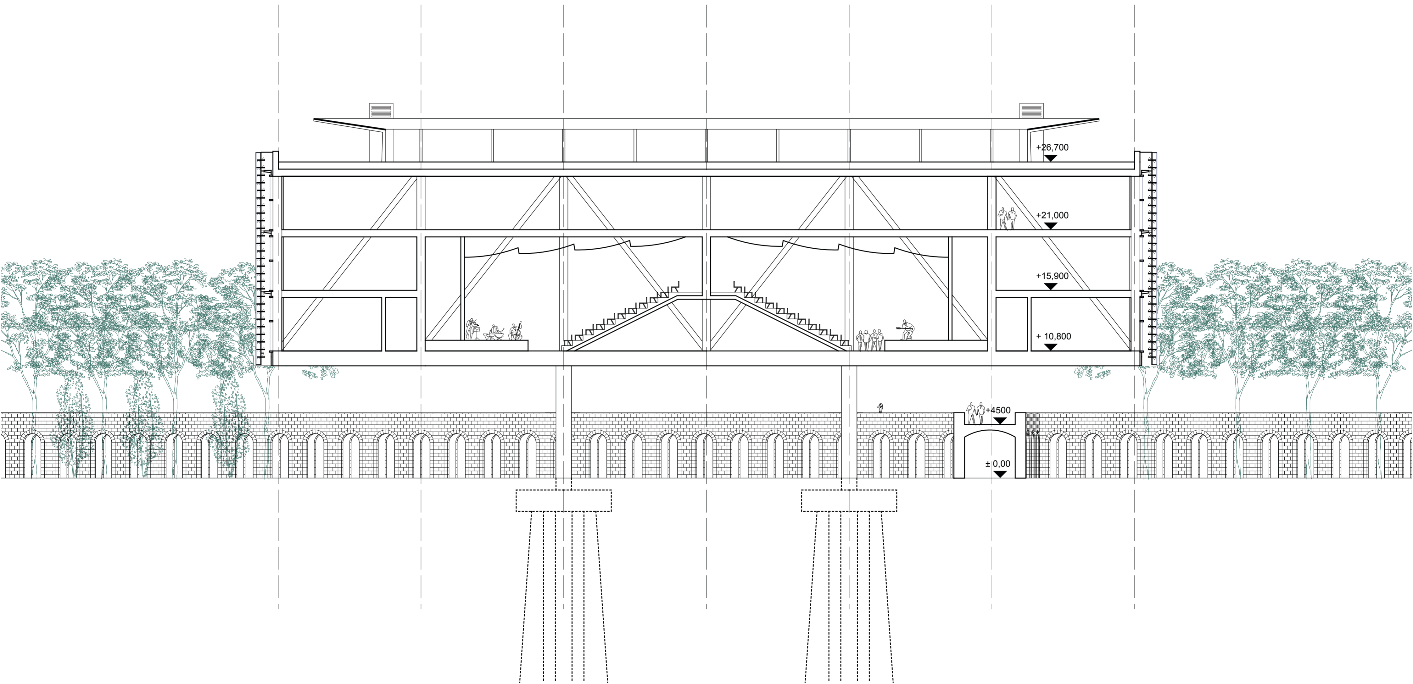
SECTION [cultural center] A-A SCALE 1:200
