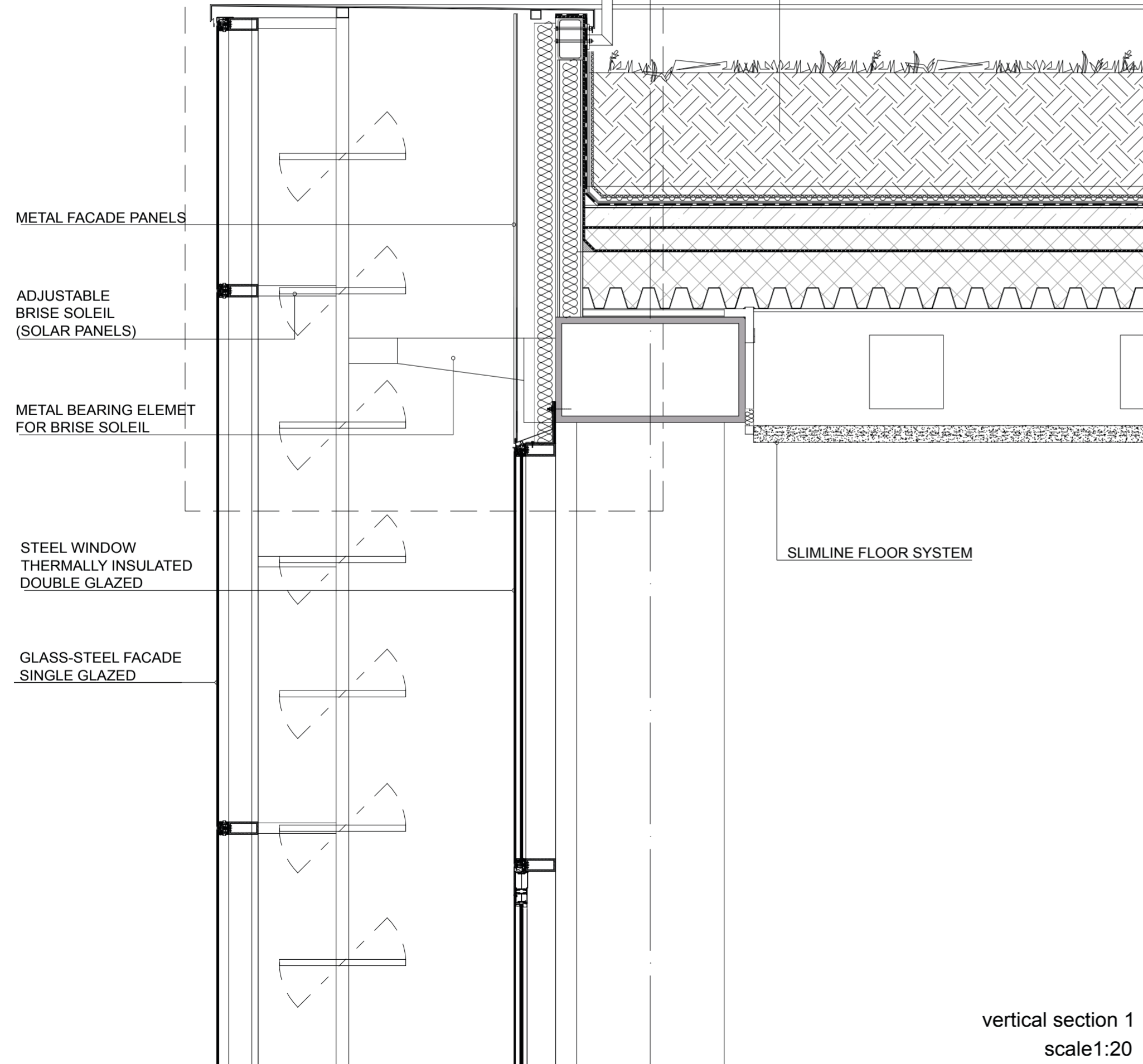
DETAIL 1 SCALE 1:10
