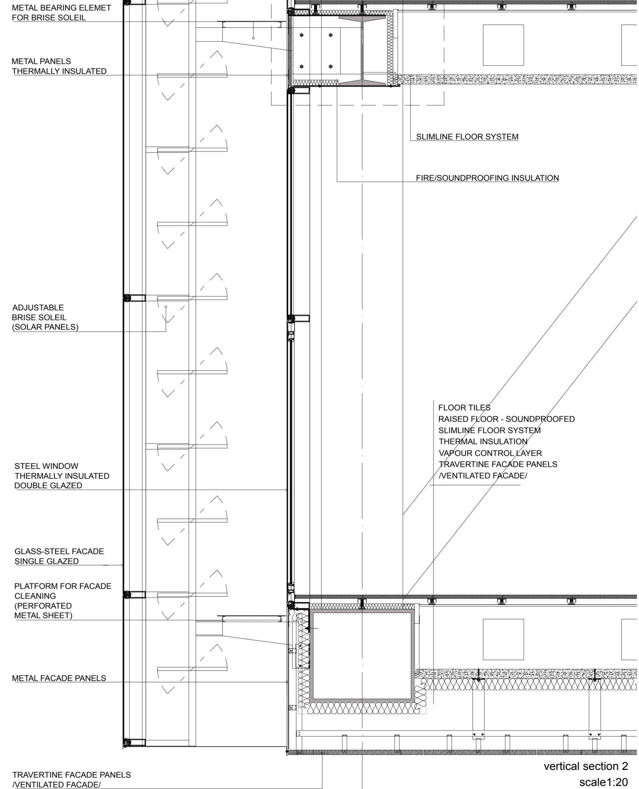
DETAIL 2 SCALE 1:5
