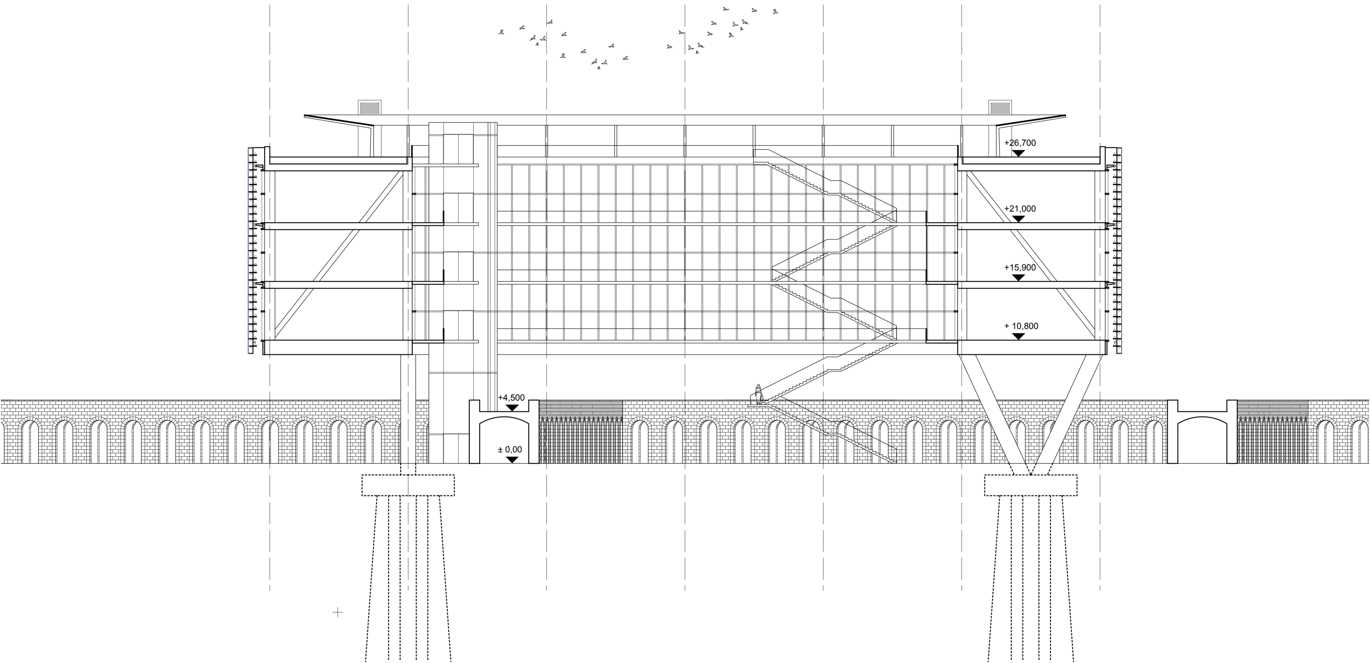
SECTION [cultural center] C-C SCALE 1:200
