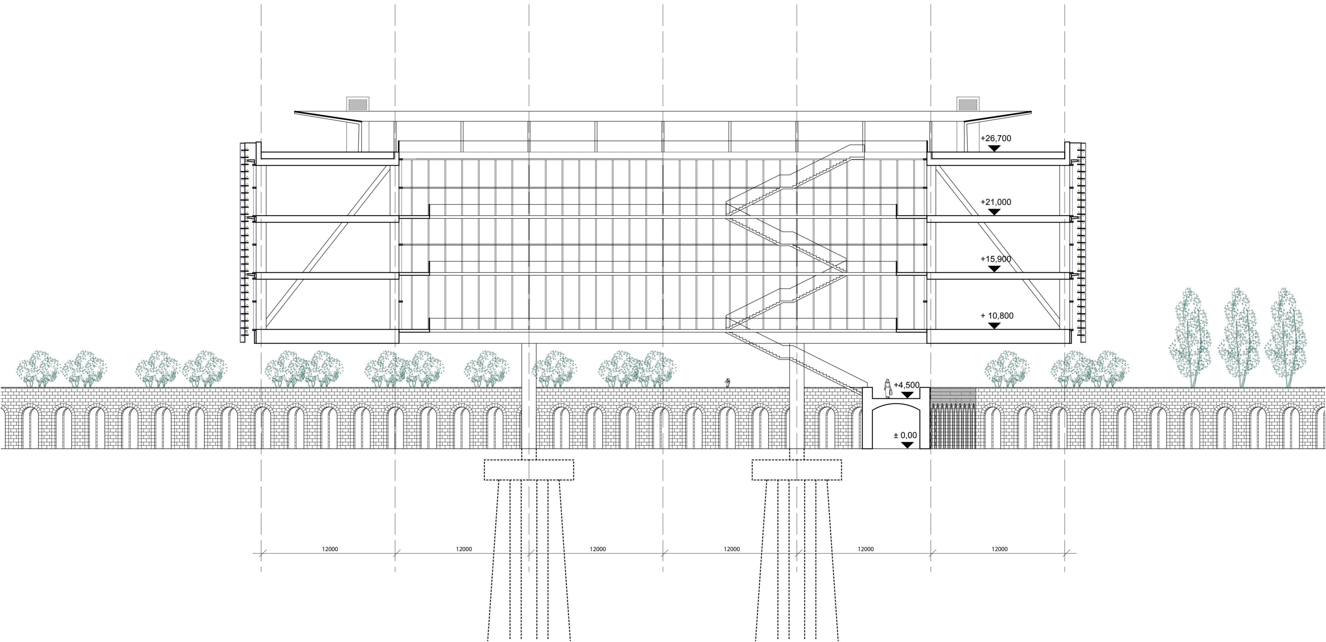
SECTION [cultural center] B-B SCALE 1:200
