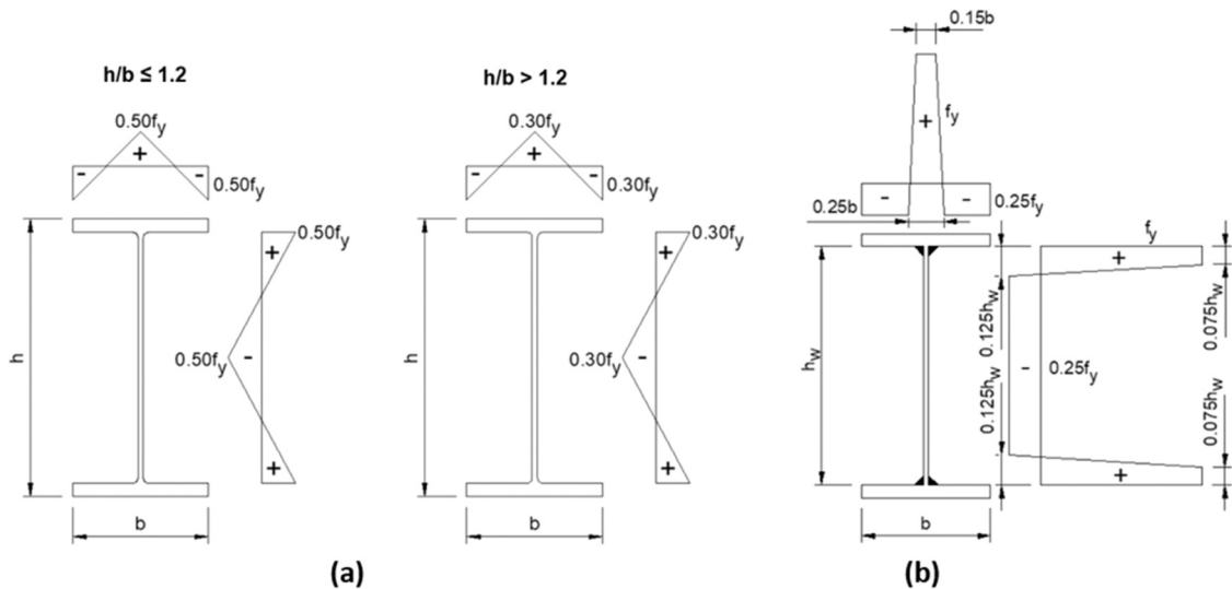
Fig. 4. Pattern of residual stresses for (a) hot-rolled and (b) welded I-sections, recommended by ECCS [46].
