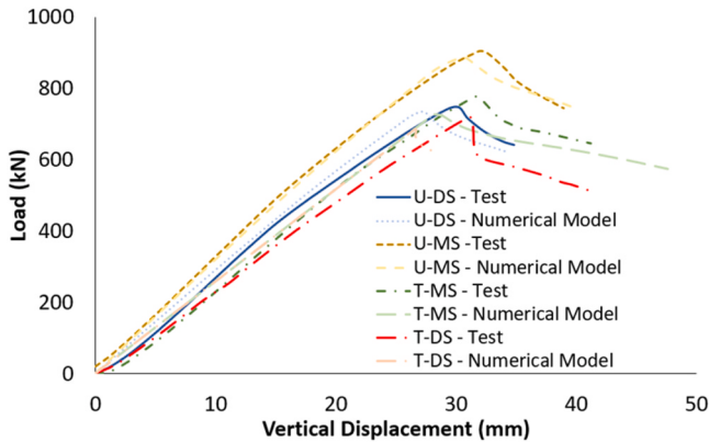
Fig. 16. Load-vertical displacement curves – displacements measured at top flange at 1.042 m from point load application (within buckling length).
