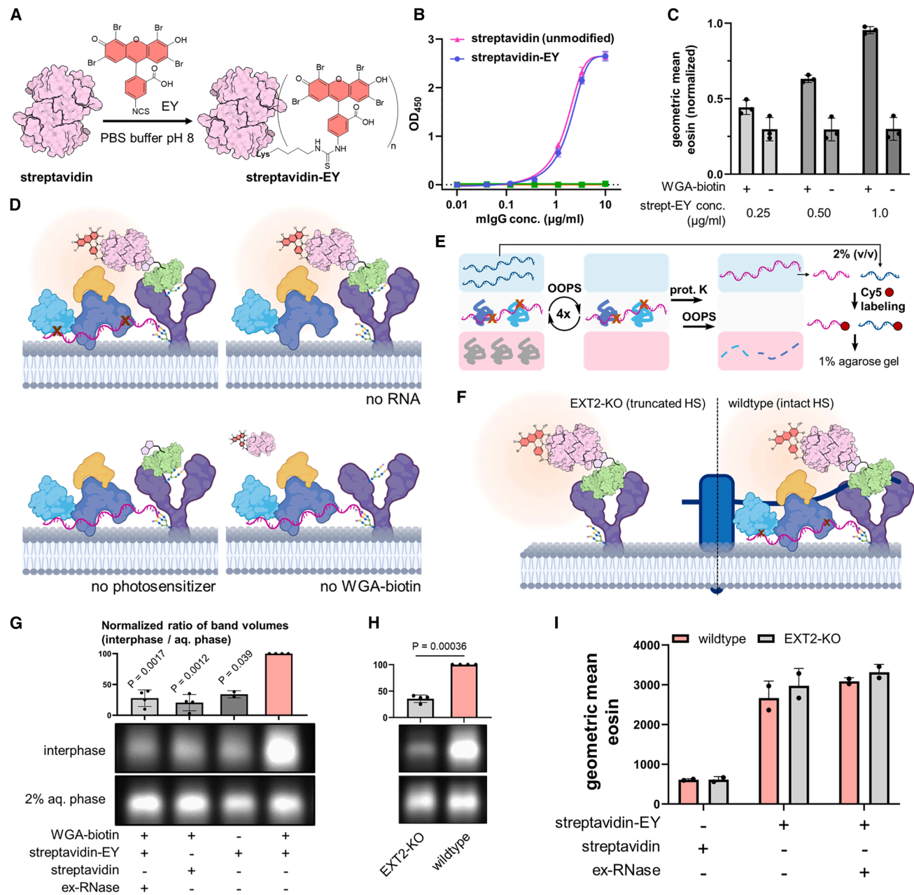
Figure 4. heprRNA HS-dependency validation by TLR7-independent cell-surface crosslinking experiments
