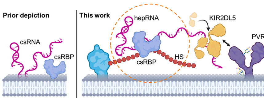
Figure 7. Molecular model of RNA cell-surface presentation
