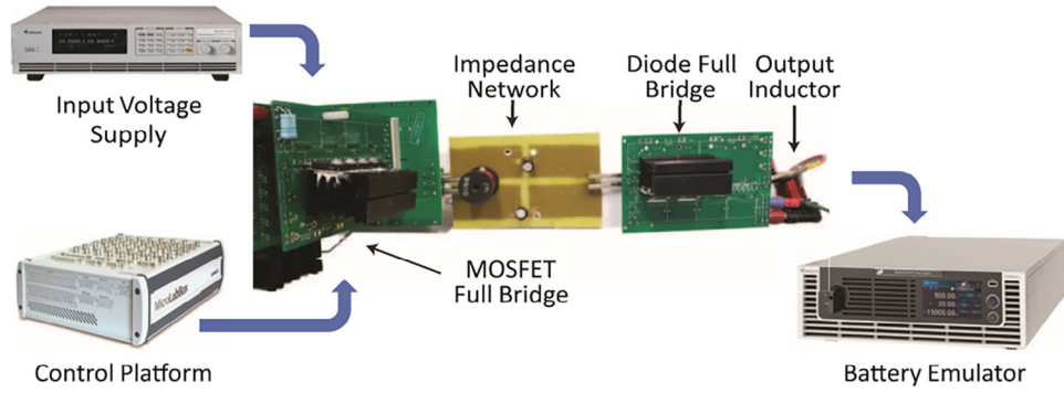
FIGURE 12 Experimental setup.
