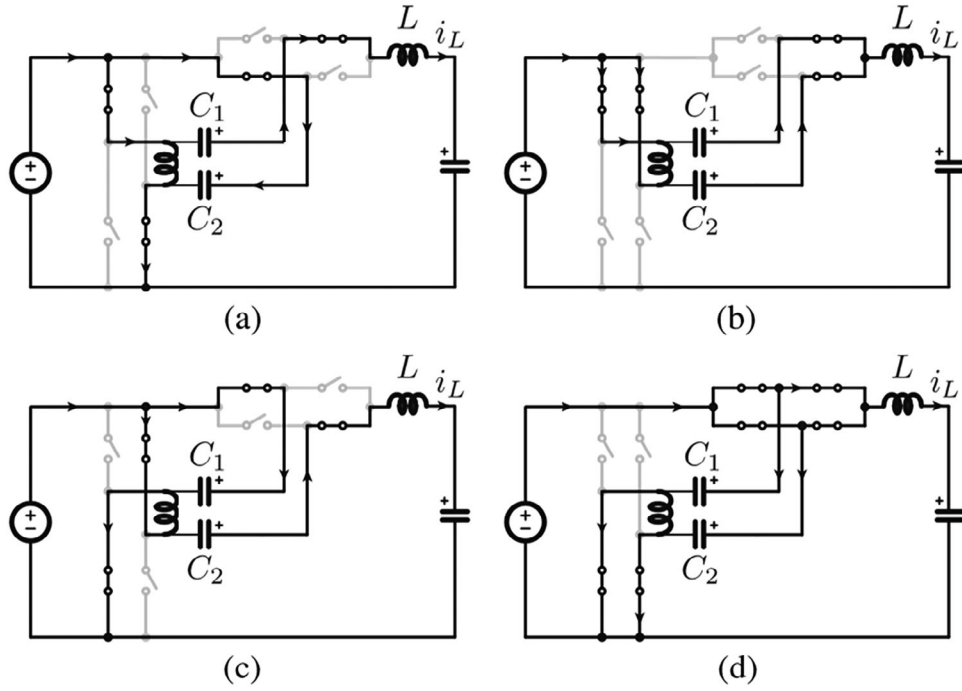
FIGURE 6 Switching states of the converter. (a) State I (S_a, S_c) = (1, 0) . (b) State II (S_a, S_c) = (1, 1) . (c) State III (S_a, S_c) = (0, 1) . (d) State IV (S_a, S_c) = (0, 0) .
