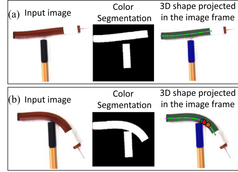
Fig. 6. An example of ground truth generation process in the case where the catheter is moving in free-space (a) and in the case of a collision upon bending to the right (b). The estimated contact points respectively by DiC and DiTE are marked by an orange and blue marker in (b), whereas the ground truth contact location is shown by a red circle.
