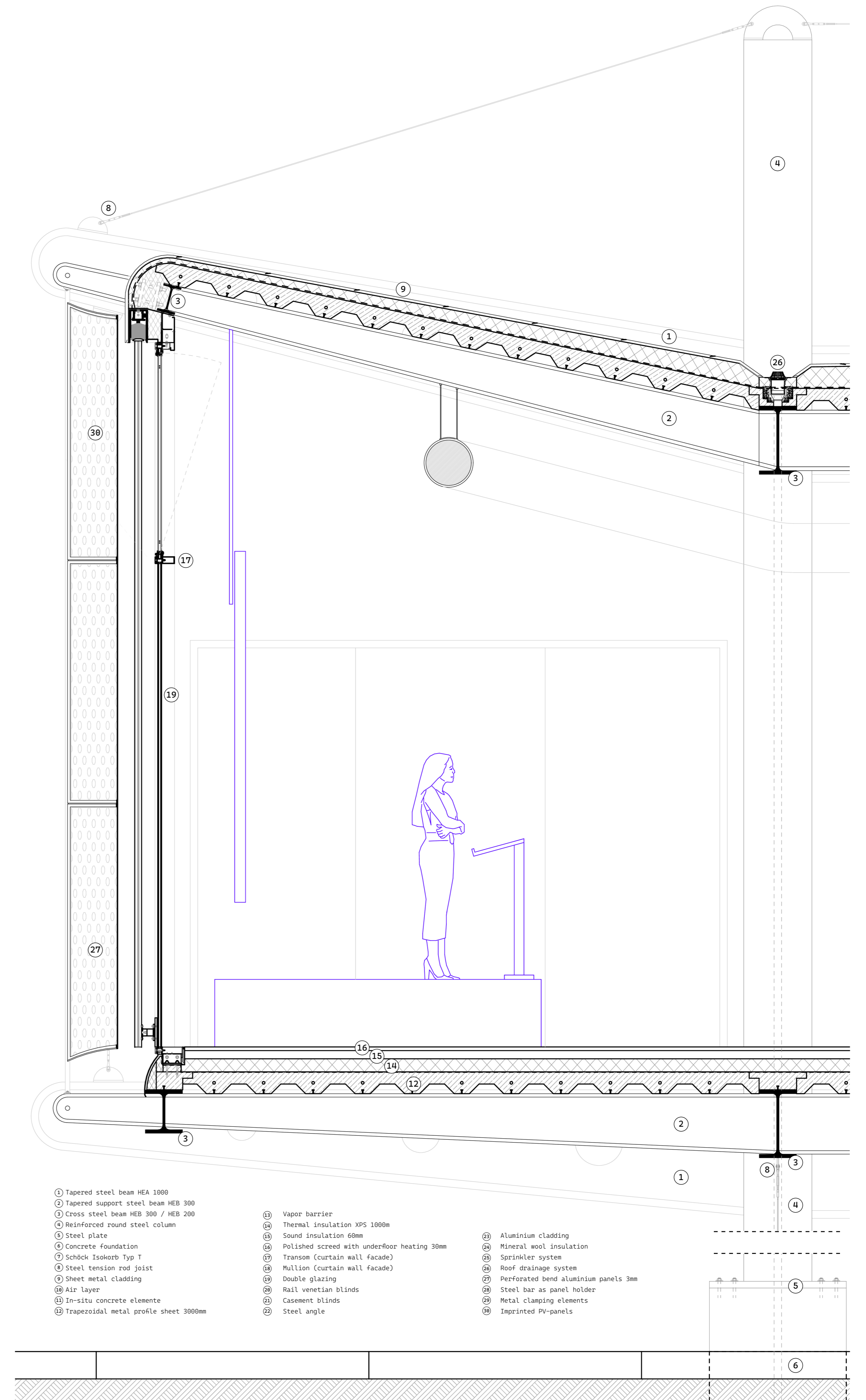
- Facade cross section - 1:20
