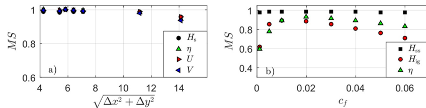
Figure 11. Grid sensitivity results for different grid resolutions (panel a), and calibration results of the friction coefficient over the reef crest to mimic frictional dissipation by the coral canopies (panel b). Panel (a) shows the skill score for bulk wave and mean flow parameters as a function of \sqrt{\Delta x^2 + \Delta y^2} relative to the finest grid ( \Delta x = 2 m and \Delta y = 2.5 m). Panel (b) shows the skill score (relative to the measurements) for the sensors over the main reef crest for three wave conditions (with a relatively energetic, moderate and weak sea-state) as a function of different friction coefficients over the reef crest.
