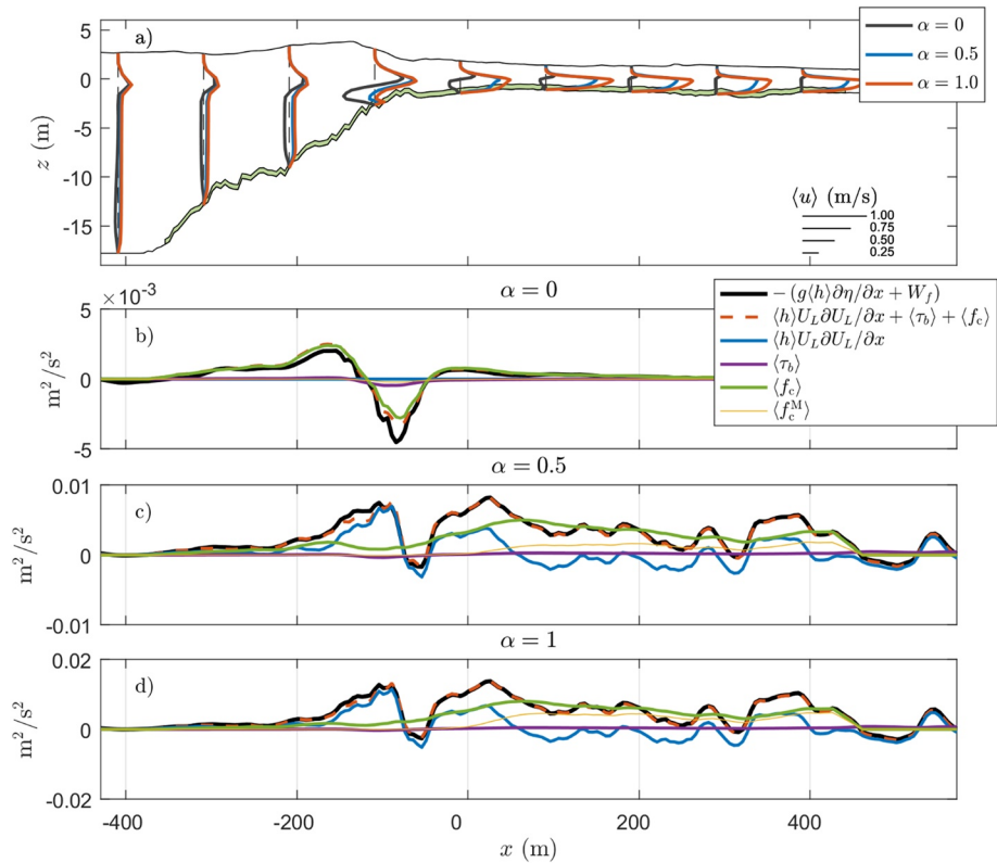
Figure 9. Mean horizontal flow profiles between the seabed and significant wave height (panel a) and the dominant terms of the cross-shore mean momentum balance (panel b–d) for a 20-layer cross-shore SWASH simulation. Results are plotted for the most energetic sea-state and for three different pump discharges ( \alpha = 0 –1 with 0.5 increment). The green shading in panel (a) indicates the canopy region in the SWASH simulation that was used to mimic the rough seabed structures. The mean-momentum terms are listed in the legend in panel (b), in which g\langle h \rangle \partial \eta / \partial x represents the pressure gradient, W_f the wave force, \langle \tau_b \rangle the mean bottom stress induced by the bare bed, \langle h \rangle U_L \partial_x U_L the advective contributions, \langle f_c \rangle the (total) mean canopy force, and \langle f_c^M \rangle the mean canopy force from the mean flow only.
