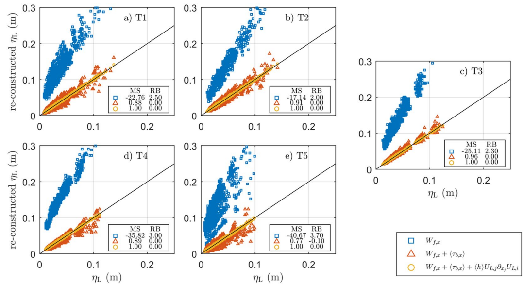
Figure 7. Comparison between the reconstructed setup inside the lagoon ( \eta_L ) based on the partial (various terms excluded) mean cross-shore momentum balance (vertical axis) and \eta_L reconstructed using all mean cross-shore momentum terms (horizontal axis). The five subplots represent a subregion of the reef-lagoon system, which combined span the full reef-lagoon system (as indicated in Figure 6a). The setup in the lagoon was taken 500 m from the shoreline, at all alongshore locations within the five subregions. The setup was reconstructed using a combination of mean cross-shore momentum terms, as indicated by the marker color and the legend in the bottom right (in which, W_{fx} represents the cross-shore wave force, \langle \tau_{b,x} \rangle the mean cross-shore bottom stress, and \langle h \rangle U_{L,j} \partial_{xj} U_{L,i} the advective contributions). Each panel includes a legend with the skill score (MS) and relative bias (RB) of each approach to reconstruct the setup.
