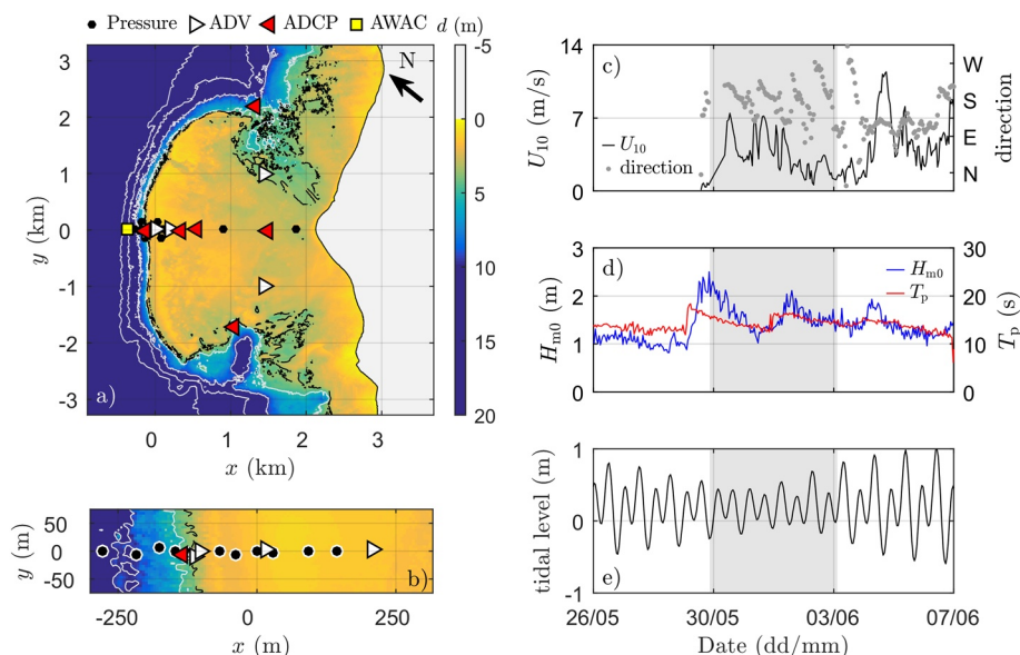
Figure 1. Overview of the model domain, instrumentation, and conditions at the considered section of the Ningaloo Reef (located at 21^{\circ}52'9.66''\text{S} , 113^{\circ}59'26.95''\text{E} ) (panel a) Plan view (panel a) and close-up near reef crest (panel b) of field instrumentation and model bathymetry with depth measured positive down. Temporal variation of the wind measured at the shoreline (panel c: wind speed, black line; and direction that the wind blows toward, gray dots), and the wave conditions (panel d: wave height, blue line; and peak period, red line) and tidal level (panel e) measured at the offshore AWAC located in about 18 m water depth. In panel (a), the dashed black indicates the 3.5 m depth contour to highlight the location of the channels, and the black line indicates the 0 m depth contour to highlight the location of the beach. The shaded gray region in panel (c)–(e) indicates the range of time that was modeled in this study, which includes two separate swell events.
