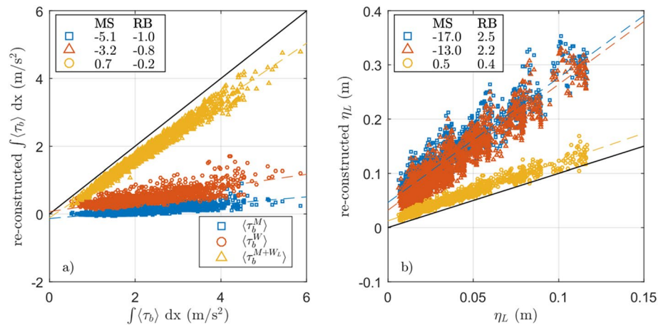
Figure 8. Comparison of the predicted and reconstructed cross-shore integrated bottom stress term (panel a) and setup inside the lagoon (panel b) for different contributions to the mean bottom stress (as indicated in the legend) and for all modeled wave conditions. Results are plotted for all cross-shore transects inside the main lagoon ( -1,800 \text{ m} \leq y \leq 1,800 \text{ m} , encompassing region T1–T5 from Figure 6). The setup inside the lagoon was taken 500 m from the shoreline, and the bottom stress was integrated from the wavemaker up to this point. The reconstructed setup (vertical axis, panel b) was computed from cross-shore integrating the mean momentum balance, including all terms, but with the mean bottom stress contribution estimated from different velocity signals (as indicated in the legend, with \langle \tau_b^M \rangle the mean bottom stress from the mean flow, \langle \tau_b^W \rangle the mean bottom stress from the (nonlinear) waves, and \langle \tau_b^{M+W_L} \rangle the mean bottom stress from the mean flow and linear waves). Dashed lines indicate a linear fit to the data for each method to reconstruct the bottom stress, and the thick black line indicates perfect agreement with the actual model prediction. Each panel includes a legend with the skill score MS and relative bias RB for each of the three methods to estimate the bottom stress.
