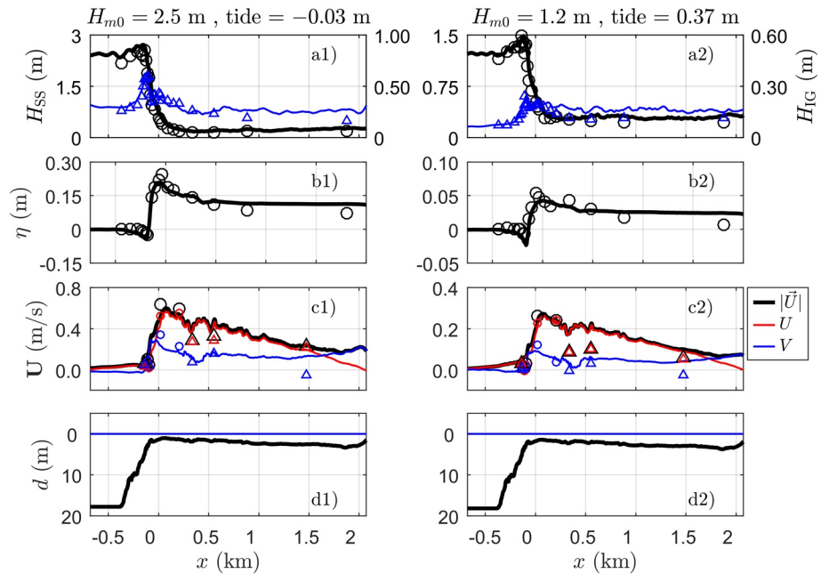
Figure 4. Model-data comparison of cross-shore variation of bulk wave and flow parameters over the central reef-transect for a relative energetic (left panels) and mild sea-state (right panels). Measured (markers) and predicted (lines) sea-swell wave height H_{SS} (panel a, thick black lines and circle markers, left axis), infragravity wave height H_{IG} (panel a, blue lines and triangular markers, right axis), wave setup \eta (panel b), mean flow velocities U (panel c), and bathymetry (panel d).
