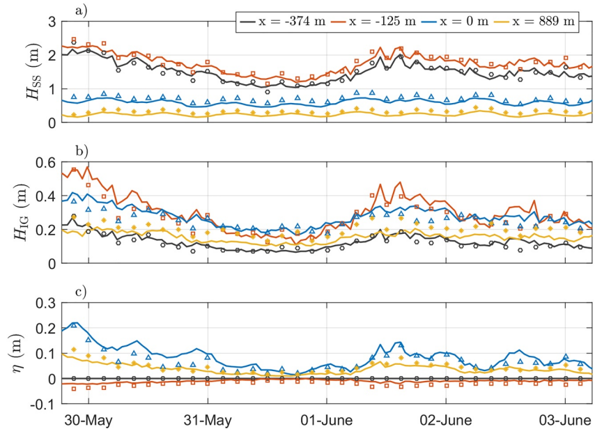
Figure 2. Measured (lines) and predicted (markers) bulk wave parameters (panel a–c) and setup (panel c) at several sensors over the central reef transect (as indicated by the line and marker color, with its cross-shore location relative to the reef crest shown in the legend). Panel (a) significant sea-swell wave height H_{SS} , panel (b) significant infragravity wave height H_{IG} , and panel (c) setup \eta .
