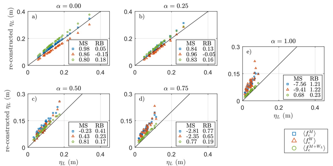
Figure 10. Comparison between the reconstructed and predicted setup inside the lagoon \eta_L for the 2DV SWASH simulations with 20 layers and a canopy flow model. The setup inside the lagoon was reconstructed using all mean momentum terms, but with different velocity signals for the mean canopy force \langle f_c \rangle (as indicated in the legend, with \langle f_c^M \rangle the mean canopy force from the mean flow, \langle f_c^W \rangle the mean canopy force from the (nonlinear) waves, and \langle f_c^{M+W_L} \rangle the mean canopy force from the mean flow and linear waves). Each panel shows the results for different discharges through the recirculating pump ( \alpha \times Q_{pump} , with \alpha = 0-1 at 0.25 increments), covering the various characteristics of natural reef systems from fringing reefs with no back lagoon ( \alpha = 0 ) to barrier reef systems ( \alpha = 1 ).
