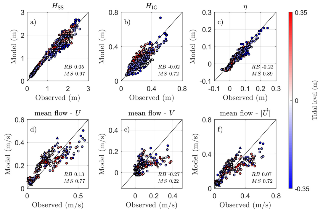
Figure 3. Model-data comparison for various bulk wave and flow parameters at all sites and for all wave conditions.
