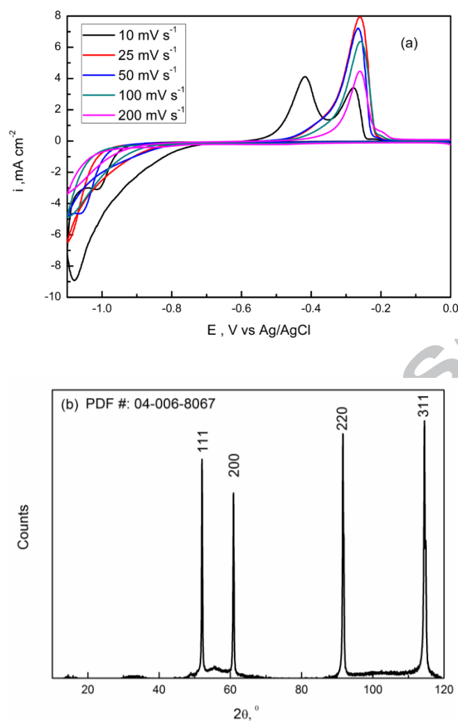
Fig. 7. (a) Cyclic voltammetry of cobalt solution at different scan rates (b) XRD pattern of the electrodeposited cobalt at 250 Am -2
