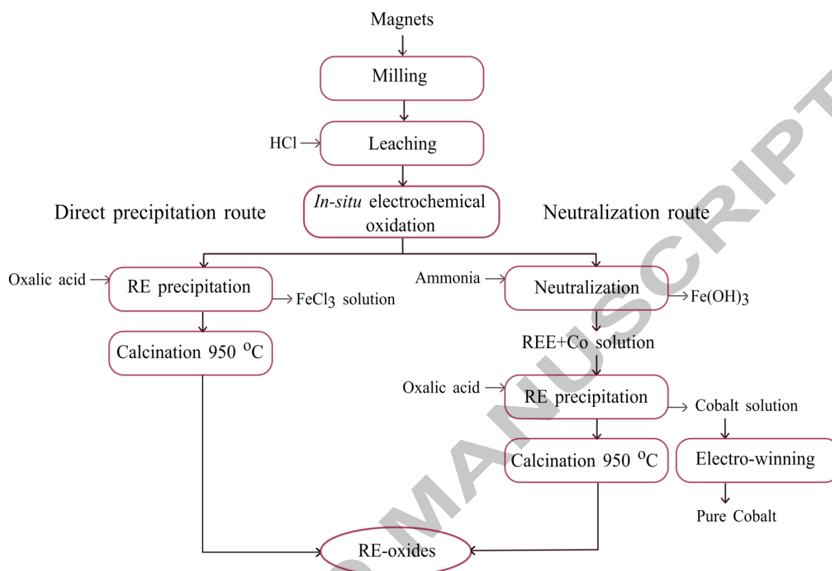
Fig. 9. Process flowsheet of electrochemical recycling of NdFeB illustrating the two different routes
