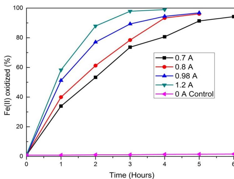
Fig. 3. Rate of Fe(II) oxidation as a function of current density (Stirring rate 550 rpm, T = 25^\circ\text{C} , C_{\text{NH}_4\text{Cl}} = 3\text{M} )
