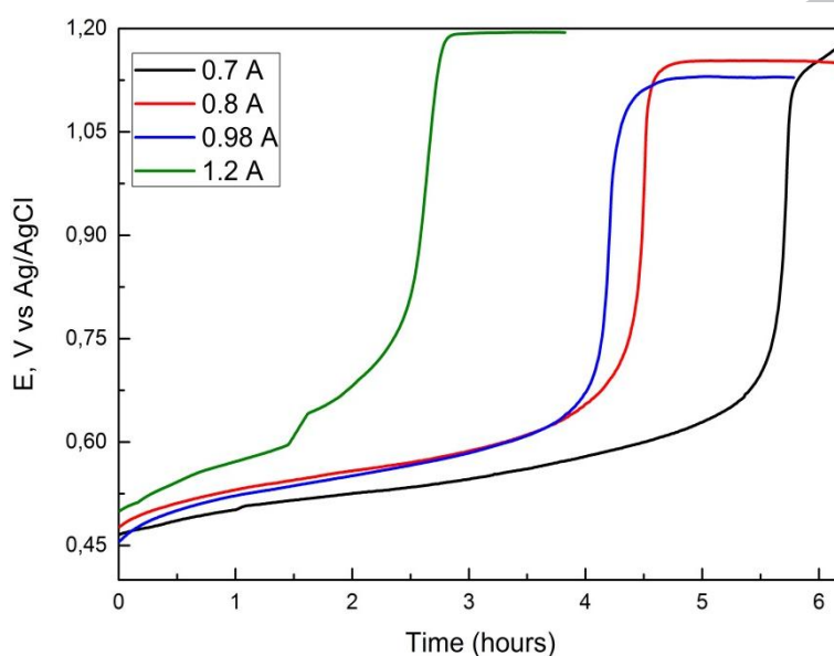
Fig. 4. Evolution of anode potential (V, vs Ag/AgCl) for different current intensities (Stirring rate 550 rpm, T = 25^\circ\text{C} , C_{\text{NH}_4\text{Cl}} = 3\text{M} )
