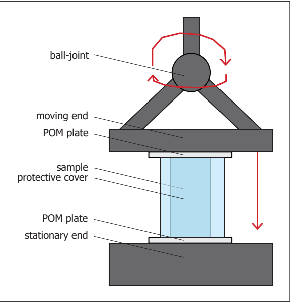
Figure 103: schematic drawing of the Toni bank set-up
