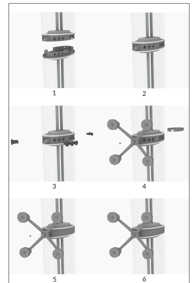
Figure 87: sequence of drawing displaying connecting two segments
