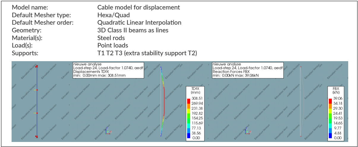
Figure 78: simulation displacement upon total failure
