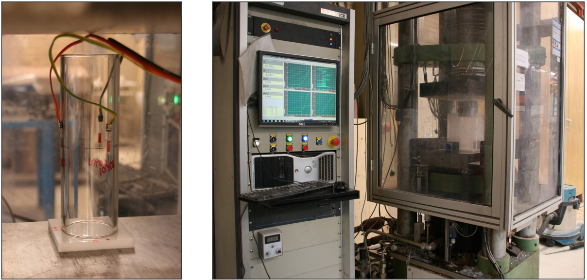
Figure 104: pictures of the strain gauges (left) and Toni bank set-up (right)
