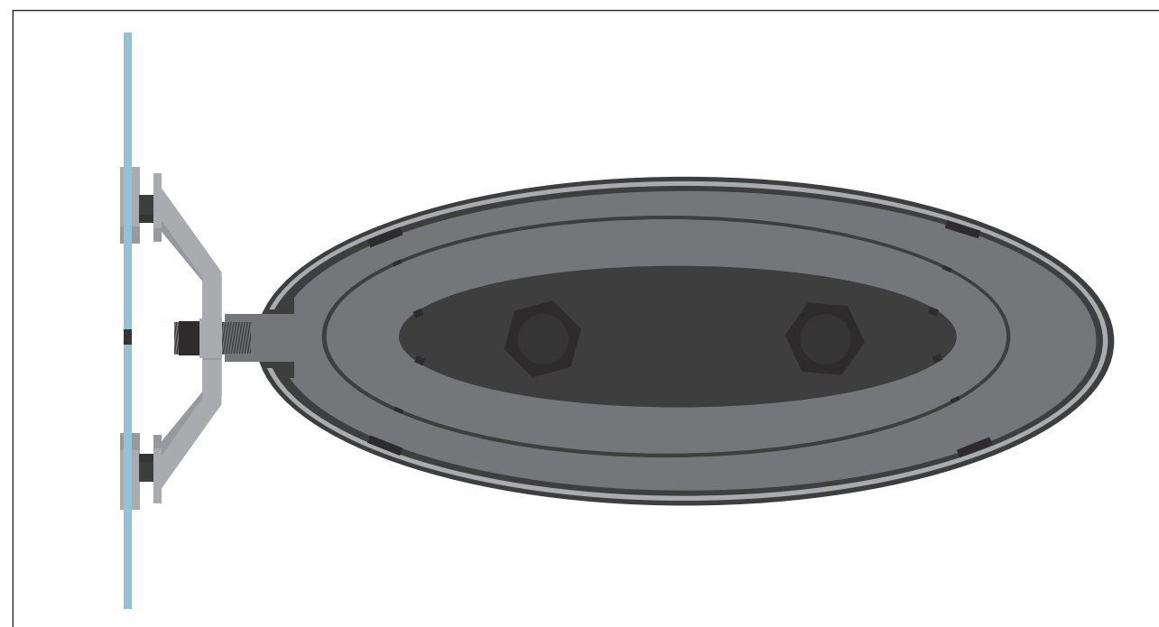
Figure 54: schematic cross section of assembled connection
