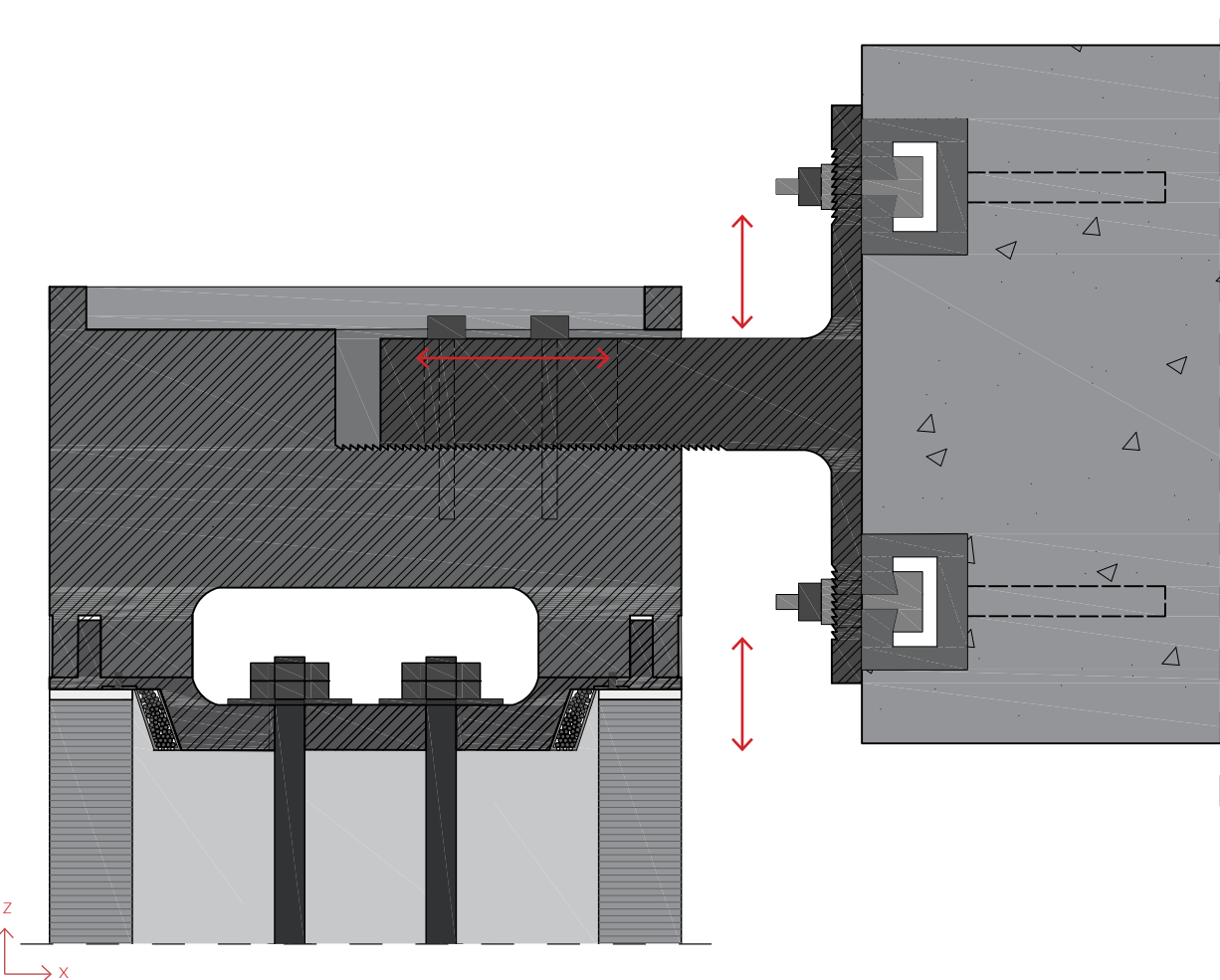
Figure 90: detail drawings of top connection
