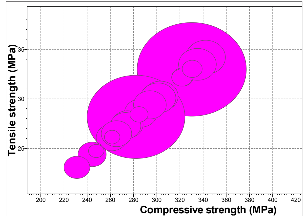
Figure 102: the tensile and compressive strengths of borosilicate glasses (CES, 2019)
