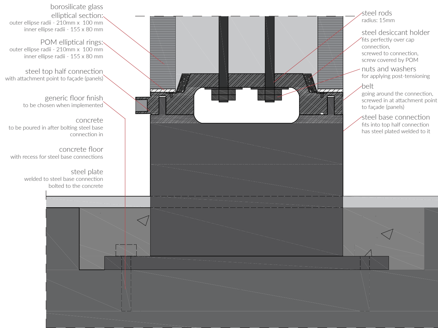
Figure 89: detail drawing of base connection
