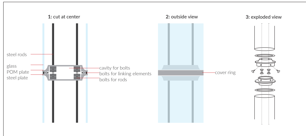
Figure 52: schematic drawings of connection principle solutions
