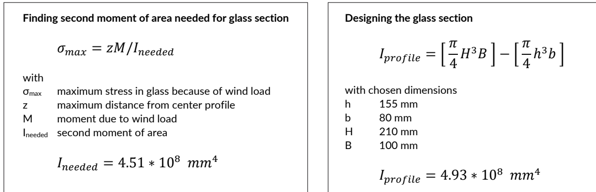
Figure 64: calculation for finding the second moment of area needed for the glass section
