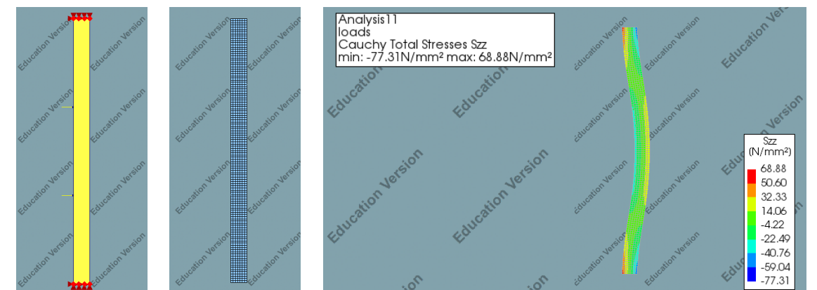
Figure 80: simulating the glass fin with the chosen dimensions of figure 99, the maximum stresses in the glass are found to be within allowable ranges. Equation from (O'Regan et al., 2015)
