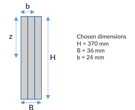
Figure 99: determining needed dimensions of glass structural fin for stress caused by moments and relevant second moments of area
