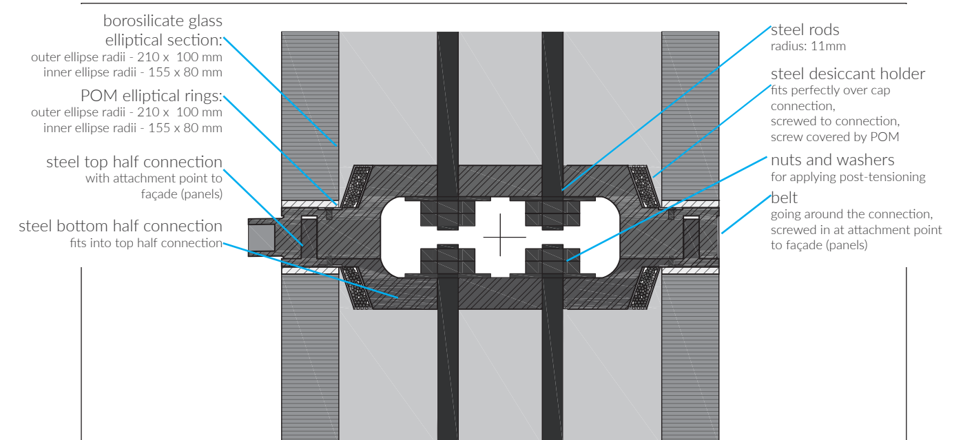
Figure 81: connection detail drawing 1:5
