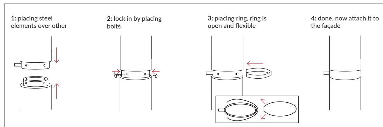
Figure 53: early sketch of installation sequence
