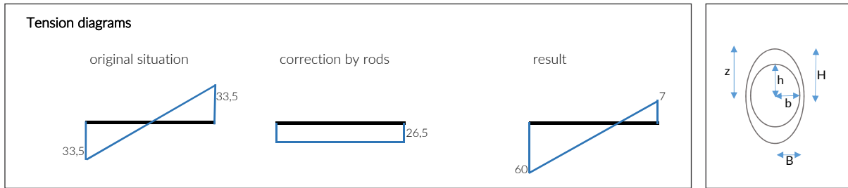
Figure 62: tension diagrams of glass with the maximum allowable compression and tension as starting point, finding the tension correction needed by the rods
