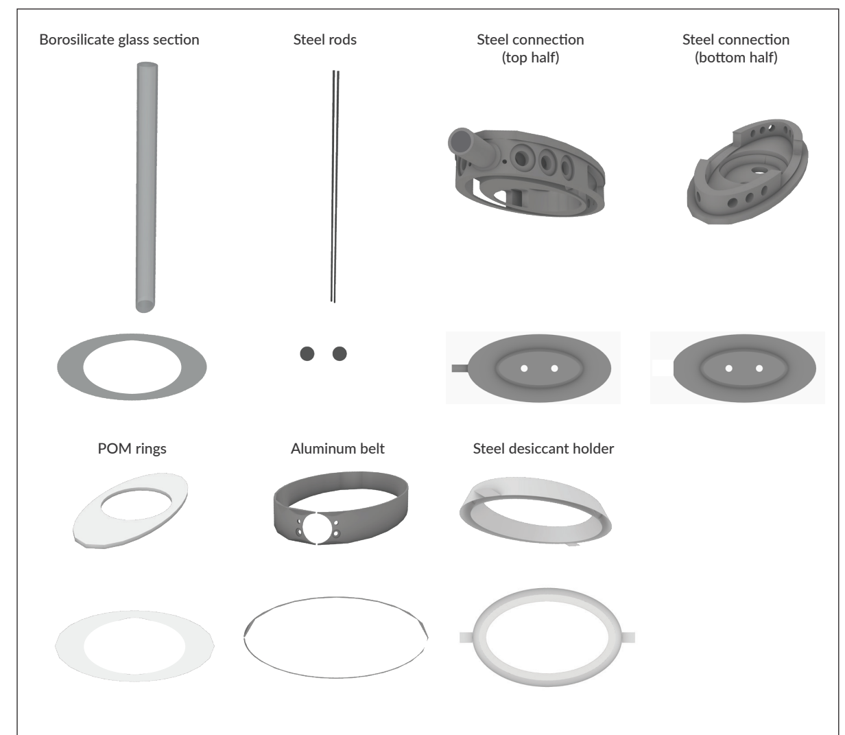
Figure 82: overview of all parts
