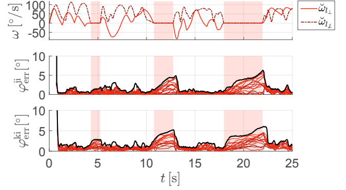
Fig. 7. Motion and estimation error for the random movement with non-observable intervals. The red areas highlight the intervals where \omega_{l_\perp}^{\text{bj}} and \omega_{l_x}^{\text{bj}} are zero.
