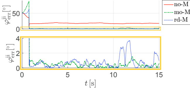
Fig. 5. Relative orientation error \varphi_{\text{err}}^{\text{ji}} between the orientation \mathbf{q}_{\text{bi}}^{\text{r}} of segment i and the orientation \mathbf{q}_{\text{bj}}^{\text{r}} of segment j .
