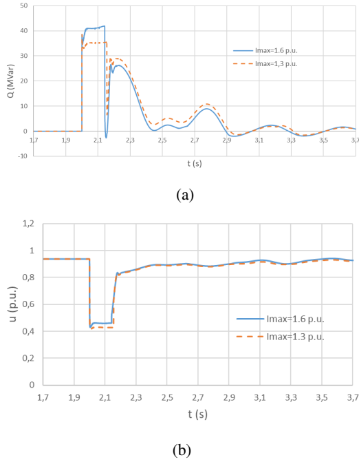
Fig. 9: Responses of the WPP03 to I_{max} = 1.6 p.u. (solid, blue) and I_{max} = 1.3 p.u. (dashed, red) (a) Reactive power injection (b) Terminal voltage
