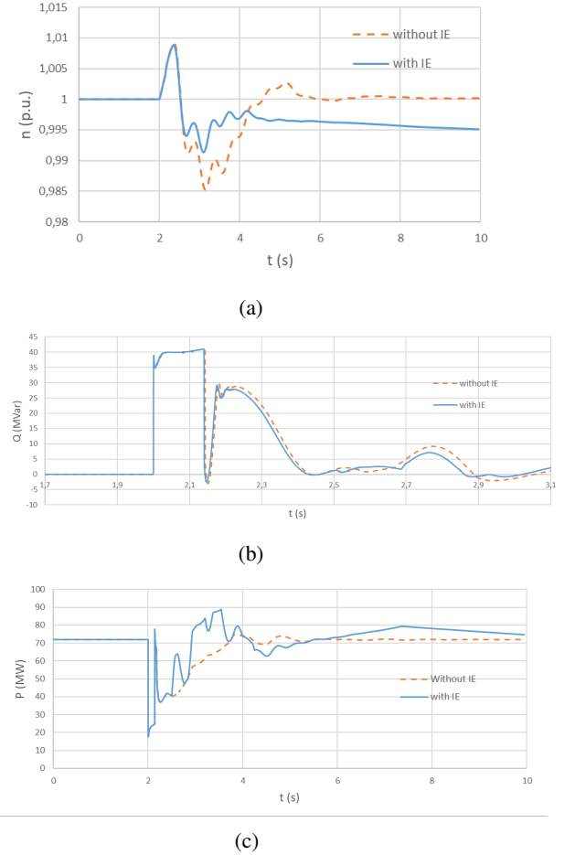
Fig. 10: Effect of different IE capability, with IE (solid, blue) and without IE (dashed, red), on (a) Speed of synchronous generator G1 (b) Reactive power injection of WPP03 (c) Active power injection of WPP03
