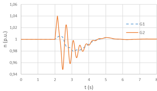
Fig. 11: Speed responses of synchronous generators G1 (dashed blue) and G2 (solid red) for the case of 78% share of FCWTGs
