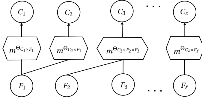
Figure 2.3: D-S valuation network representation of the knowledge-based fault diagnosis problem. The variables F_1 till F_\ell indicate the presence or absence of the different system faults f_1 till f_\ell , the variables C_1 till C_z represent the diagnostic features, and the valuations (multivariate mass functions) m^{\Theta_{C_1 \times F_1}} , m^{\Theta_{C_2 \times F_1}} , m^{\Theta_{C_3 \times F_2 \times F_3}} , and m^{\Theta_{C_z \times F_\ell}} express the (uncertain and incomplete) relationships between the respective variables.
