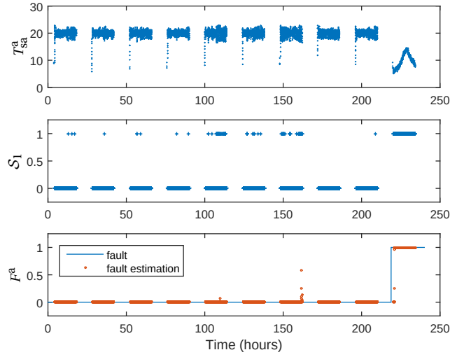
Figuur 4.10: AHU fault diagnosis example 1 for case study 1.
