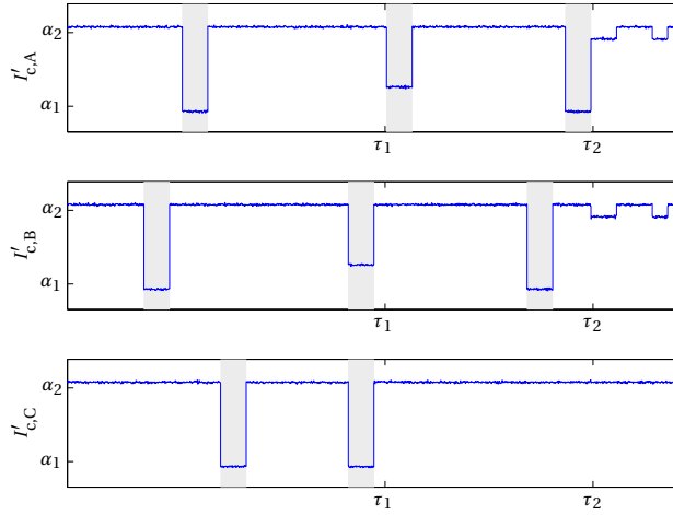
Figuur 3.12: Monitoring signals of sections A, B, and C.
