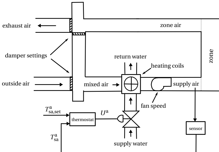
Figuur 4.5: Schematic overview of an AHU.
