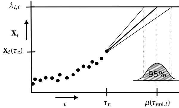
Figuur 6.1: Illustration of the prognostic result at \tau = \tau_c . For \tau \leq \tau_c , the degradation measure X_i(\tau) is known. For \tau > \tau_c we predict the behavior of the degradation measure based on its previous values and the fault-specific parametric model (linear here). From this prediction and the failure threshold \lambda_{l,i} , the distribution of the estimated failure time in mode l , p(\tau_{eol,l}) , can be determined.
