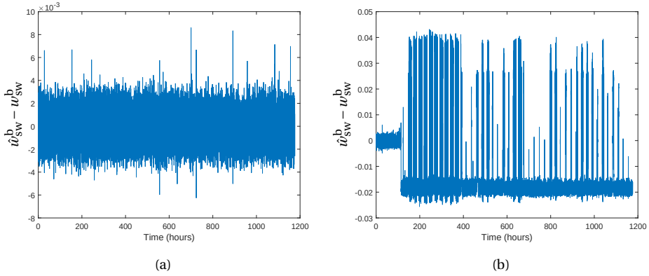
Figure 4.13: Time behaviors of \hat{u}_{sw}^b - w_{sw}^b : (a) healthy AHU valve; (b) stuck AHU valve.
