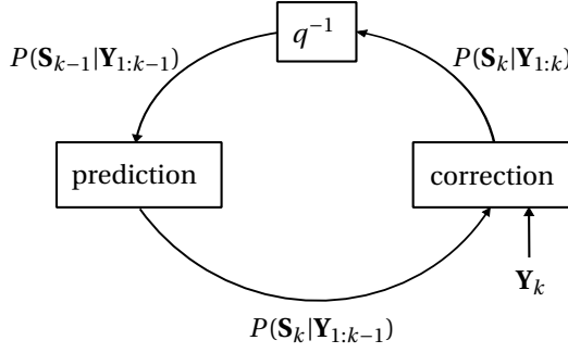
Figuur 5.3: Bayesian filtering. At each time step k , first, the state is estimated based on the model (prediction step). Next, this estimate is updated based on the current measurements \mathbf{Y}_k (correction step).
