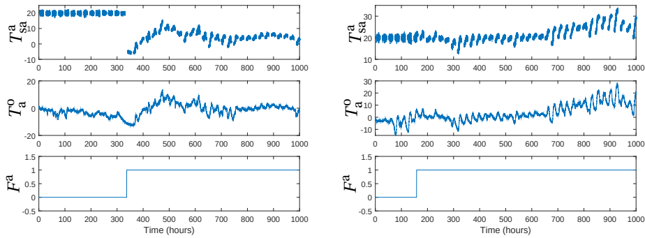
Figuur 4.9: Possible behaviors of T_{sa}^a corresponding to a stuck heating coil valve. Left: the valve got stuck during the night in a cold period. Right: the valve got stuck during the day while the outside temperature is increasing.
