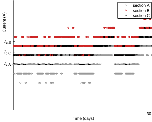
Figure 3.9: Current measurements of sections A, B, and C when the section is free.
