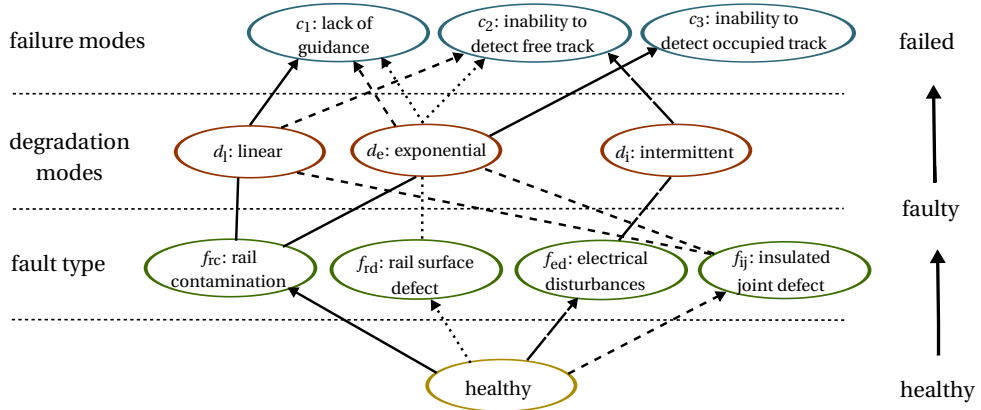
Figuur 5.2: Visualization of the relationships between the faults, degradation modes, and failure modes of a railway track.
