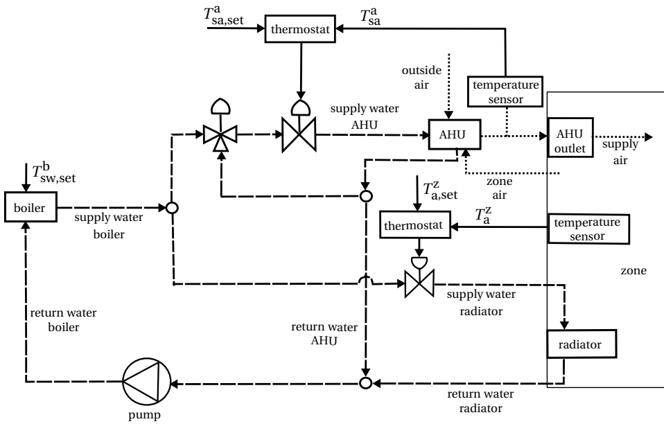
Figuur 4.4: Overview of the considered HVAC system. Dotted lines represent air flows, dashed lines represent mass flows, and solid lines represent signals.
