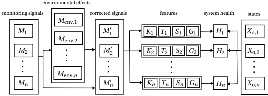
Figuur 3.2: Schematic overview of the proposed knowledge-based fault diagnosis approach.
