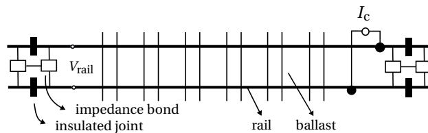
Figuur B.1: Overview of a railway section and the corresponding track circuit.
