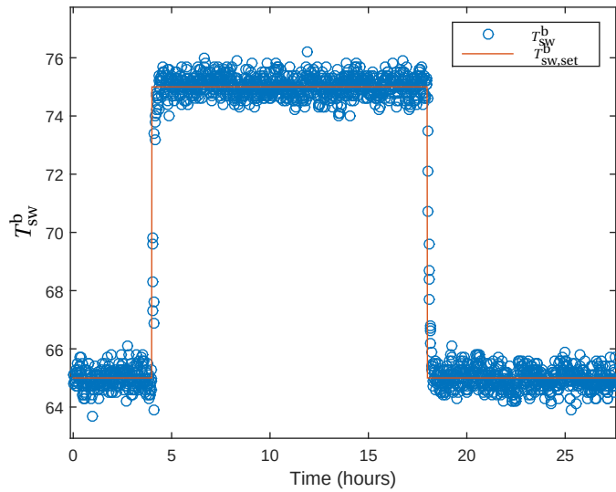
Figure 4.14: Daily behavior of T_{sw}^b .
