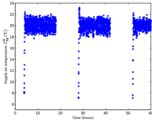
Figure 4.7: Typical daily behavior of the supply air temperature with a sample step of one minute. Note that during the night, the AHU supply air temperature is not controlled.
