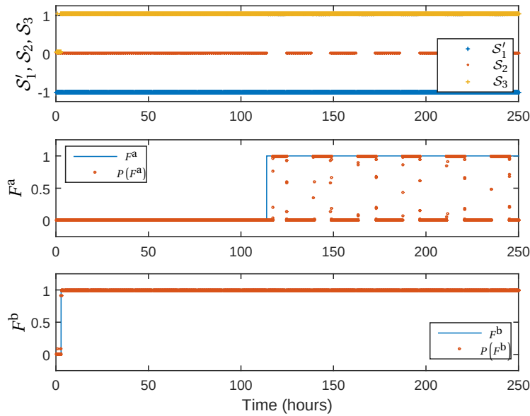
Figuur 4.15: Boiler and AHU fault diagnosis example for case study 2.
