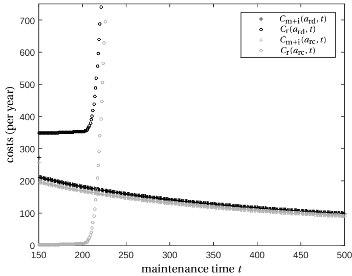
Figuur 6.10: Cost components for the different maintenance strategies ( \tau = \tau_{150} ).
