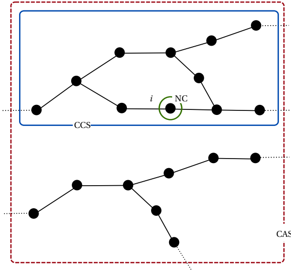
Figuur 3.7: Division of the sections (track circuits) in a railway network for the fault diagnosis of section i .
