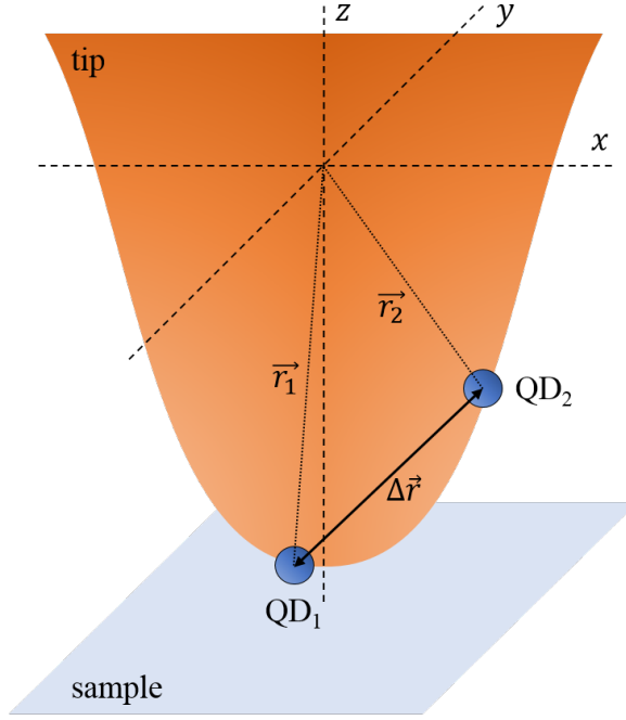
Figure 6.10: Multiple quantum dots on the tip. If multiple quantum dots exist on the apex of our STM tip, they will have a certain relative distance \Delta \vec{r} . Their relative position might be found by comparing the response of the resonances to the position of the tip over a known surface geometry with a known electric field.
