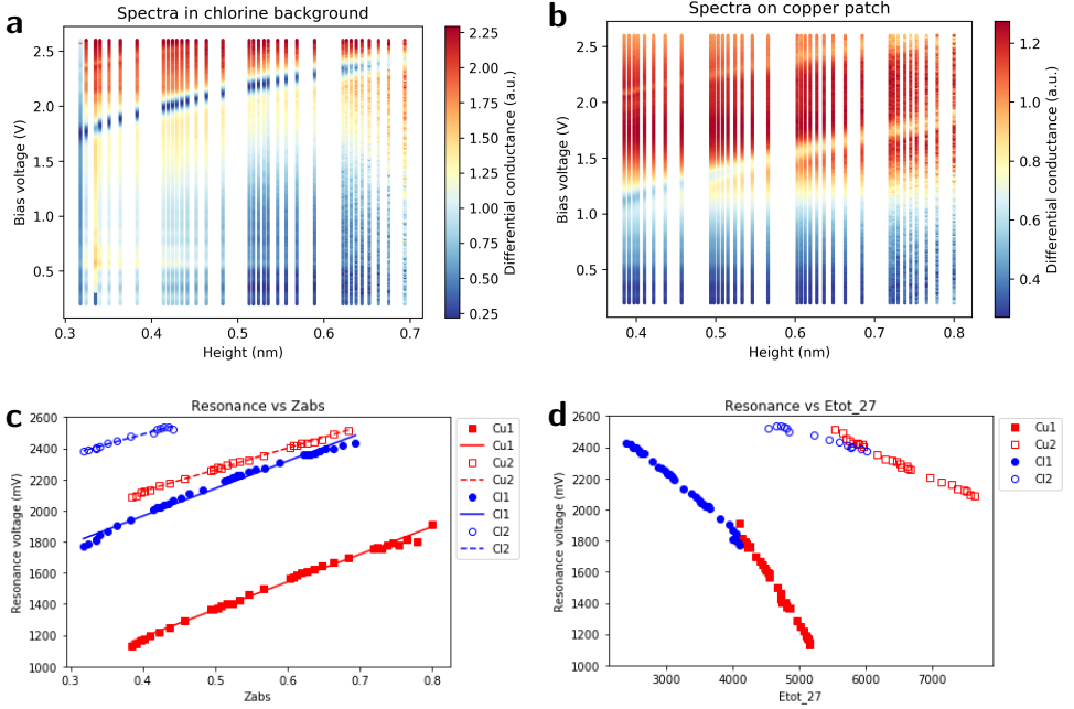
Figure 6.11: Behaviour of the quantum dot resonance on the chlorine background and on a copper patch. a , Each point in a normalised dI/dV spectrum (colour scale) as a function of the bias voltage and its absolute height, where spectra have been taken on the chlorine background for multiple set-point currents, i.e. tip heights. b , Same as in (a) , but in the centre of an 11 \times 11 copper patch. c , The resonance voltage of the two resonances in each spectrum, as a function of the absolute height. Red squares are on the copper, blue circles on the chlorine background. Filled markers are the main resonance at lower voltage, open markers are the second resonance at higher voltage. Linear fits have been drawn through each of the four sets. d , For each of the points in (c) , the total electric field has been calculated from the tip field E_t = V/z and the simulated sample field E_s(z) by E_{tot} = E_t + c \cdot E_s , with c = 0.27 . Both the first resonances (filled markers) and the second resonances (open markers) line up with this factor.
