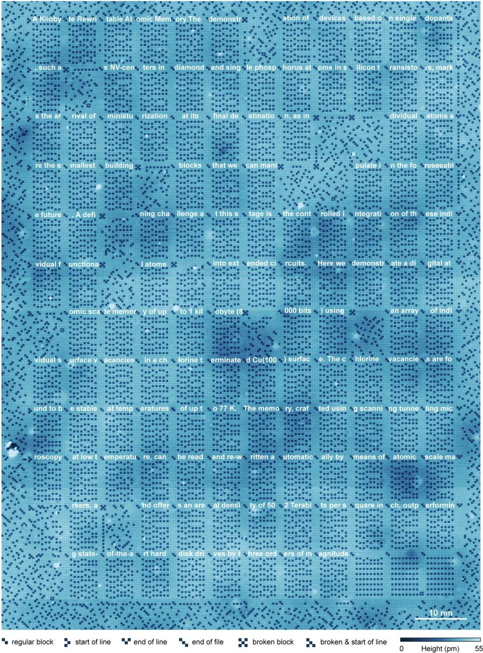
Figure 3.5: Kilobyte atomic memory. STM image (96×126 nm, I = 2.00 nA, V = +500 mV, T = 1.5 K) of the memory shown in Figure 3.3, extended to 1,024 bytes (8,192 bits), written to the abstract of an early version of [42]. The areal density of this modified memory is 506 terabits per square inch.
