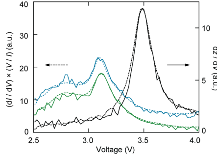
Figure 4.3: Comparing dz/dV (solid lines) and dI/dV \times V/I spectra (dashed lines). Black, blue and green correspond respectively to the bare Cl/Cu(100) substrate and two different vacancies within the stripes lattice.
