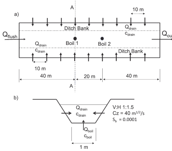
Figure 2.2: a. Schematization of the test polder ditch (not to scale) for the first scenario, 10 m drainage spacing, 1 m bed width, 1:1.5 side slope, Chezy coefficient 40 \text{ m}^{1/2}/\text{s} and bottom slope 0.0001 [-] with flushing discharge ( Q_{flush} ), outflow discharge ( Q_{out} ), groundwater drain exfiltration discharge ( Q_{drain} ) and concentration ( c_{drain} ), locations of the two boils and two locations used in controller design that are 40 m and 60 m downstream of the flushing inlet, b. Cross section of the ditch (A-A in (a)) with drain exfiltration discharge ( Q_{drain} ) and concentration ( c_{drain} ), boil discharge ( Q_{boil} ) and concentration ( c_{boil} ).
