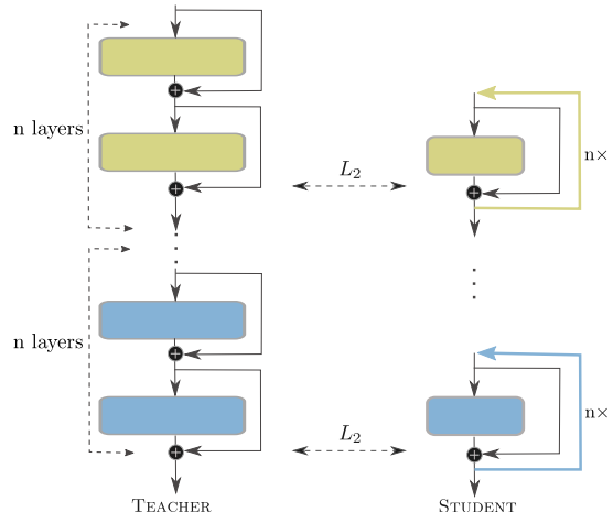
Fig. 1. Multiple residual layers in the teacher network (left) are mapped to a single layer in the student network (right) through recurrence. The L_2 measures similarity between networks, and similar colors correspond to similar layers between networks. Note the reduction in layer parameters.
