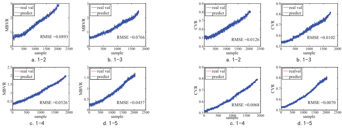
(a) Prediction results of MBVR
