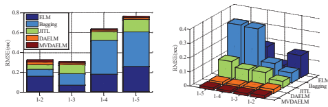
Fig 6. Comparison of modeling prediction results for PD that the proposed algorithm MVDAELM can always obtain the best prediction results in the soft sensor experiment. The comparison between the DAELM prediction results and the MVDAELM prediction results shows that after the introduction of multi-view learning, the prediction results are more stable and the error is reduced. Figure 4 shows the prediction results of three mill load parameters for domain adaptive learning with the operating condition 1 as the source domain.
