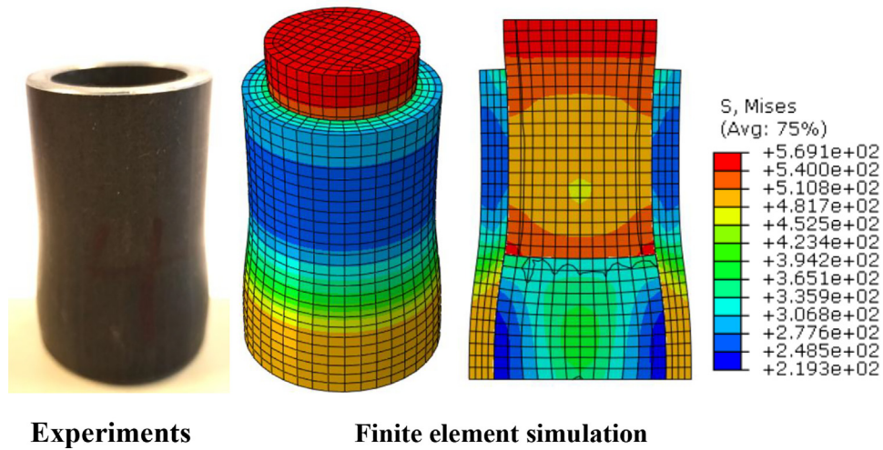
Figure 23.16 Deformation comparisons between FEM and experiments of confined resin.
