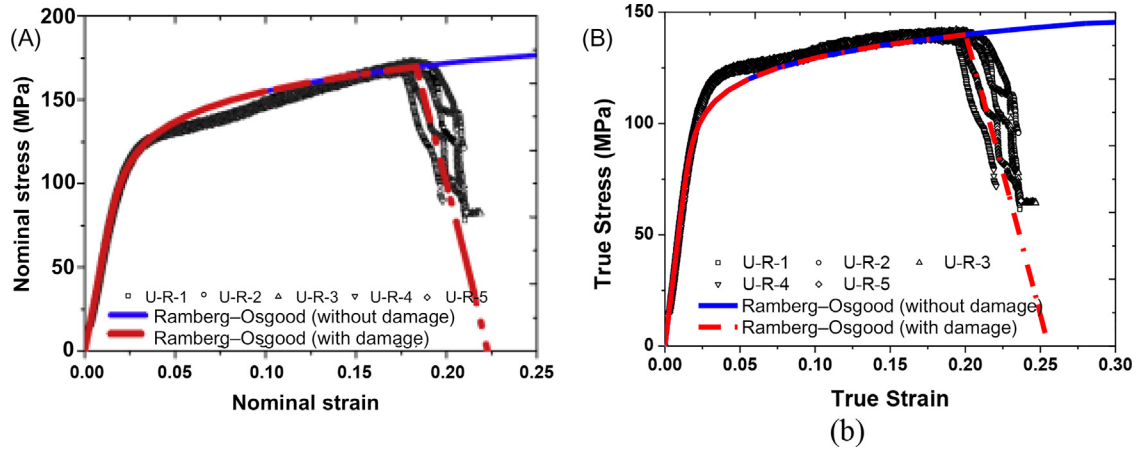
Figure 23.6 Stress–strain relationship of unconfined resin specimens: (a) Nominal stress versus nominal strain and (b) True stress versus true strain.
