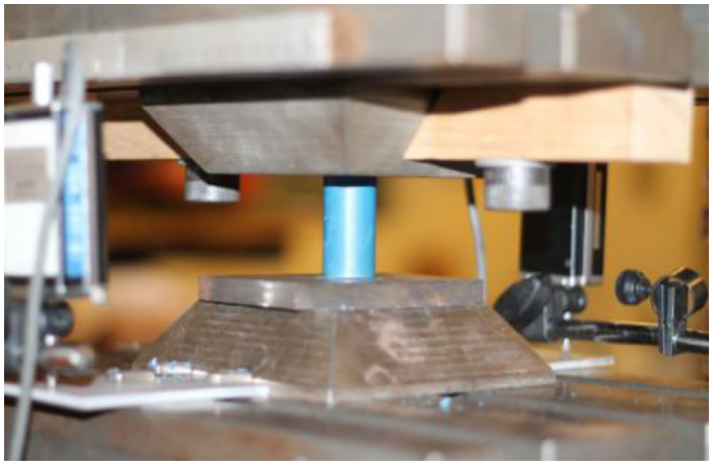
Figure 23.5 Experimental set-up.
