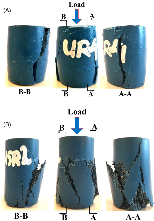
Figure 23.8 Typical failure mode for resin (A) and steel-reinforced resin (B).
