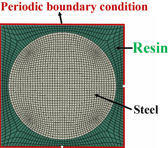
Figure 23.17 Unit cell of steel-reinforced resin.
