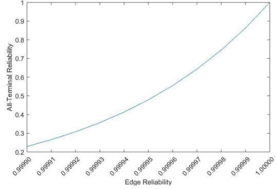
Figure 2. The all-terminal reliability of the texel gas distribution network for different uniform edge reliabilities
