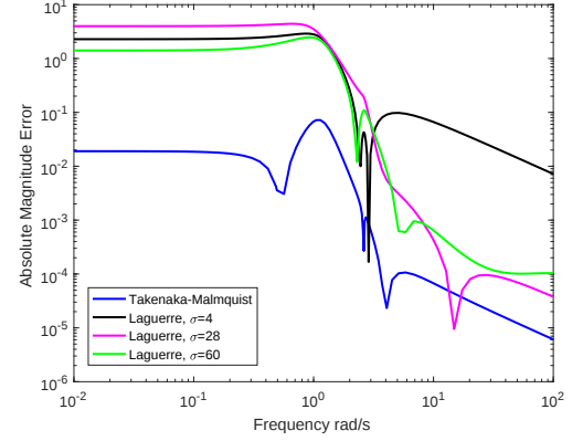
Fig. 4. Identification performance in terms of the frequency response error |G(j\omega) - \hat{G}(j\omega)| with \hat{G}(j\omega) being the estimated frequency response.
