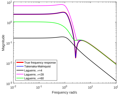
Fig. 3. Bode frequency responses of the original and identified systems. Note that the frequency-response curve of the Takenaka-Malmquist method overlaps with the true frequency-response curve.
