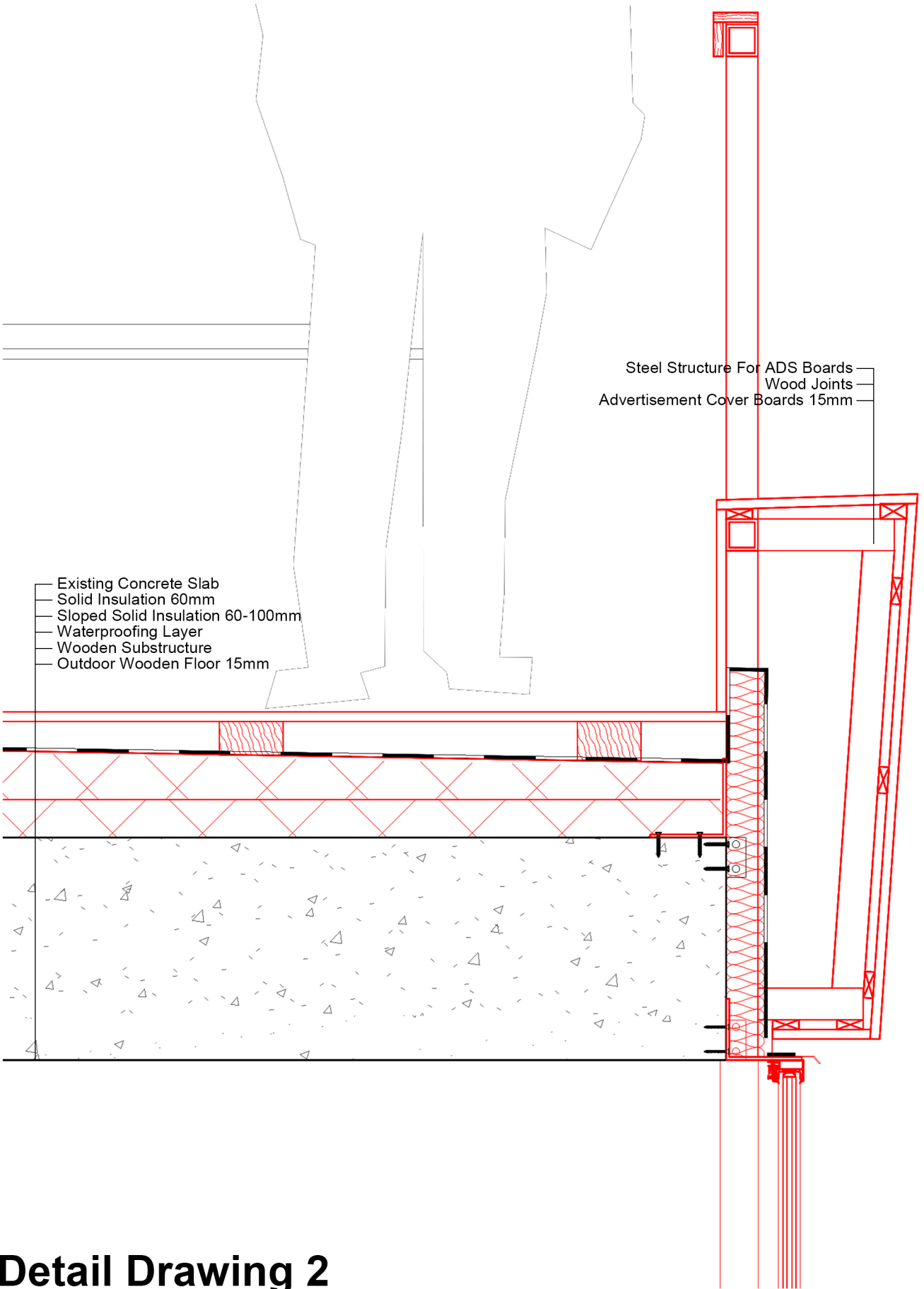
Detail Drawing 2
