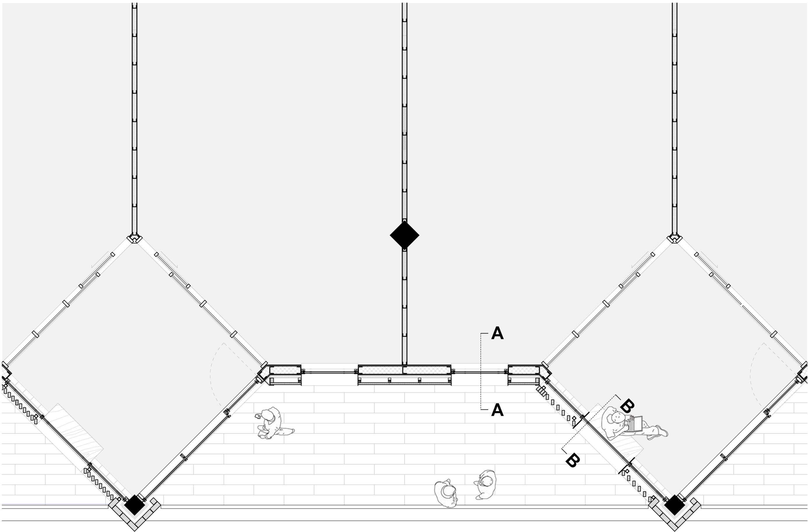
Horizontal Section Detail Drawing
