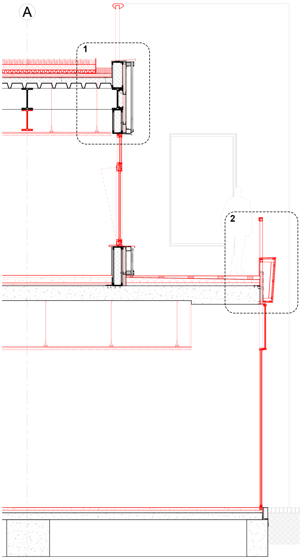
A-A Section Drawing
