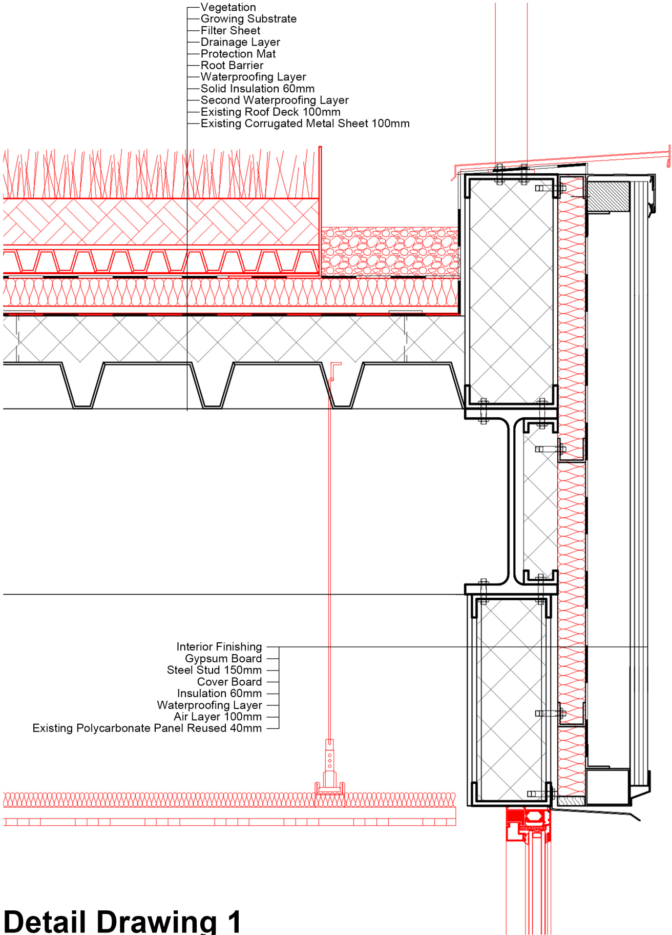
Detail Drawing 1
