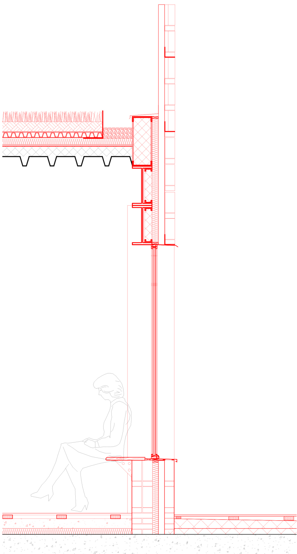
B-B Section Drawing
