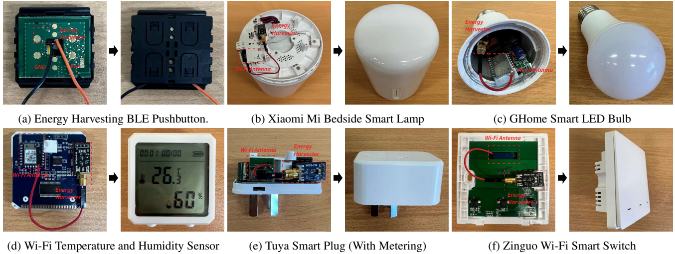
Figure 25: Integrating AppListener into commodity IoT device with energy harvesters and Wi-Fi antennas as is shown in Table 5
