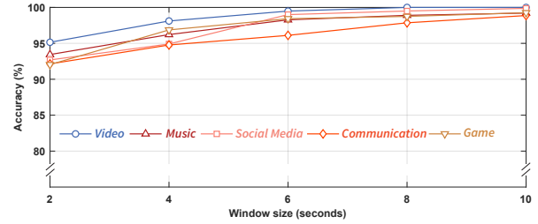
Figure 16: Analysis of the impact of sliding window size.
