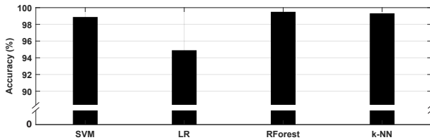
Figure 8: Accuracy (%) of different classifiers in identifying the category of the app.
