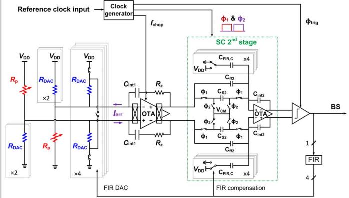
Figure 3.6.2: Simplified system block diagram.
