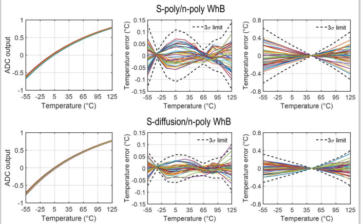
Figure 3.6.4: Sensor characteristic (left); temperature inaccuracy after a 1st-order-fit and a 5th-order systematic nonlinearity removal (middle) or a correlation-based 1-pt trim (right).
