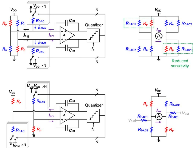
Figure 3.6.1: Conventional multi-bit CTΔΣ readout of a Wheatstone bridge sensor (top left); proposed readout scheme with an embedded RCM DAC (bottom).
