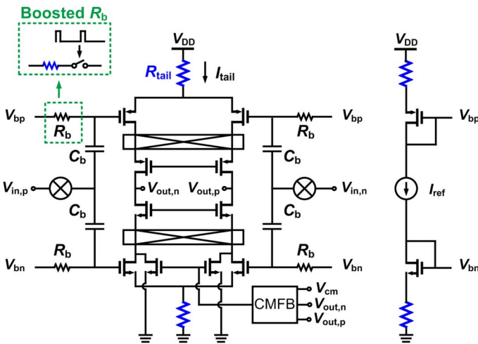
Figure 3.6.3: Simplified diagram of the chopped capacitively-coupled 1st-stage OTA with robust biasing and tail resistor linearization.
