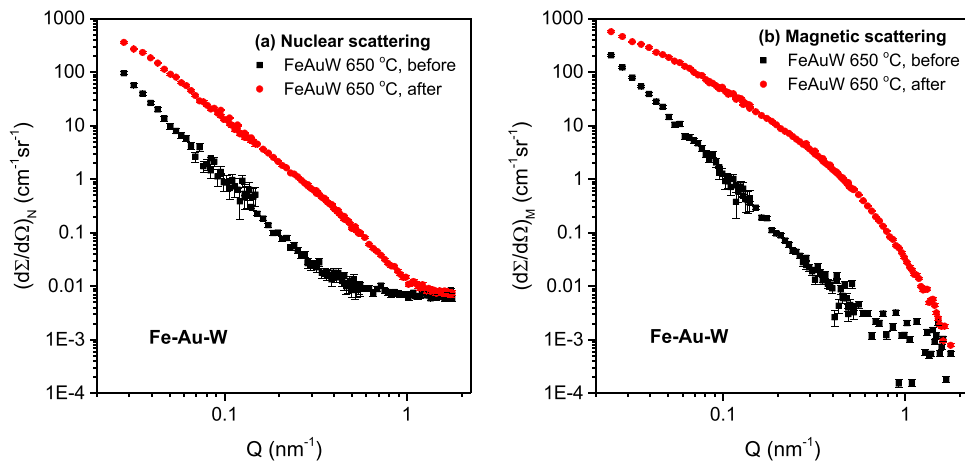
Fig. 5. SANS profiles for the Fe-Au-W alloy measured at room temperature before and after 12 h of aging at 650 °C showing: (a) nuclear scattering (d\Sigma/d\Omega)_N(\mathbf{Q}) for \alpha = 0^\circ , (b) magnetic scattering (d\Sigma/d\Omega)_M(\mathbf{Q}) for \alpha = 90^\circ .
