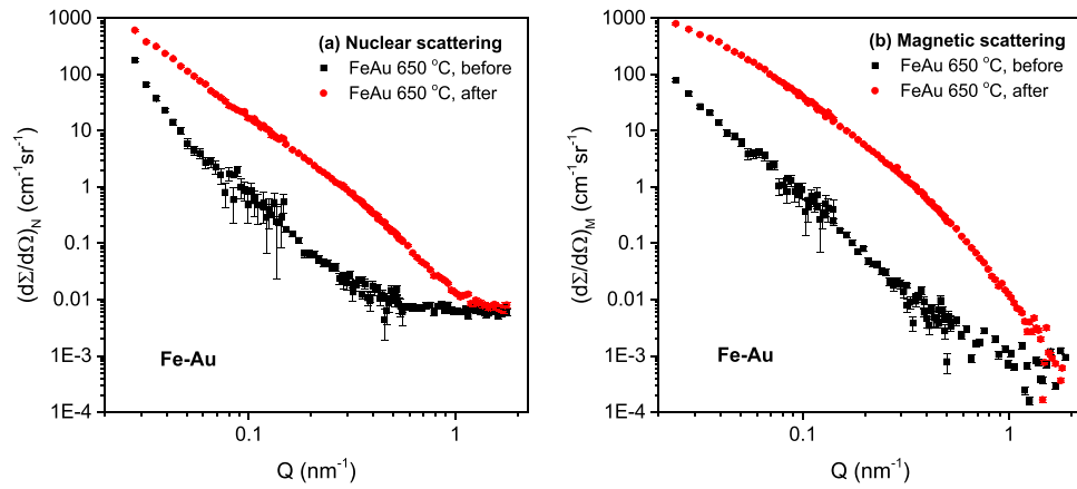
Fig. 6. Q -dependent SANS for the Fe-Au alloy before and after aging for 12 h at 650 °C for (a) nuclear scattering (d\Sigma/d\Omega)_N(Q) for \alpha = 0^\circ , (b) magnetic scattering (d\Sigma/d\Omega)_M(Q) for \alpha = 90^\circ .
