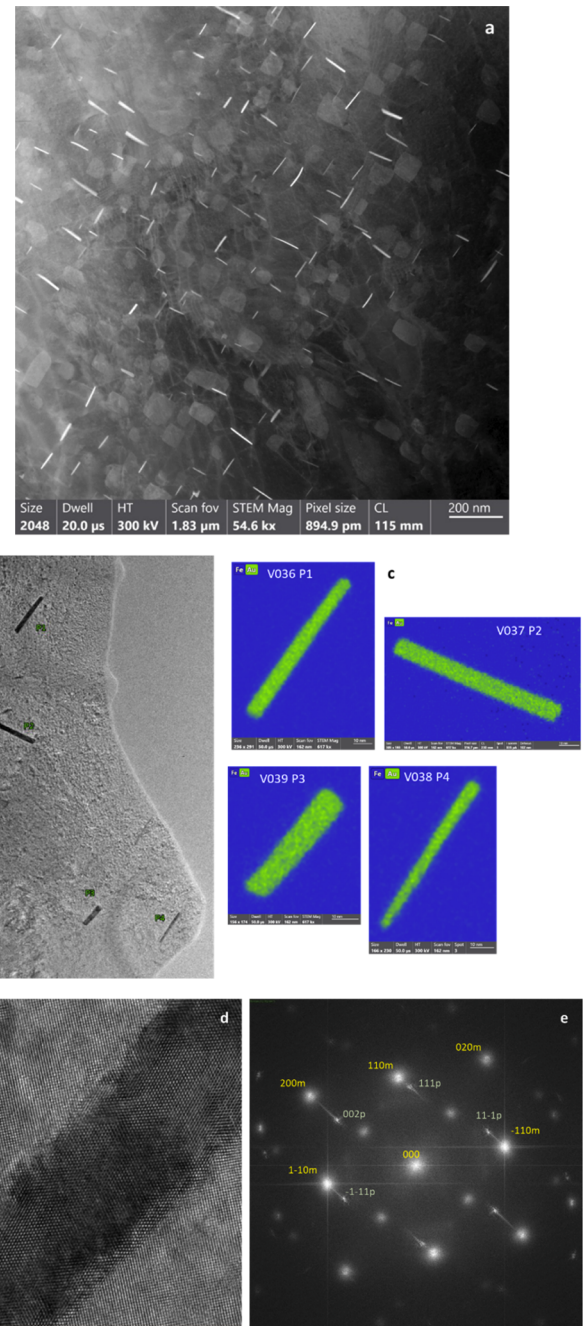
Fig. 2. STEM and TEM images of the cold-rolled homogenised Fe-Au alloy after 12 h of aging at a temperature of 650 °C. Au-rich plate-shaped precipitates are clearly visible in (a). The Au-rich precipitate in (b) was analysed to map the (c) Au concentration. The precipitate contains about 60 at.% Au. (d) High resolution image of the precipitate and the surrounding matrix. (e) FFT image of (d) confirming the previously reported orientation relation between the bcc matrix and the fcc precipitate for Fe-Au alloys [15,17].
