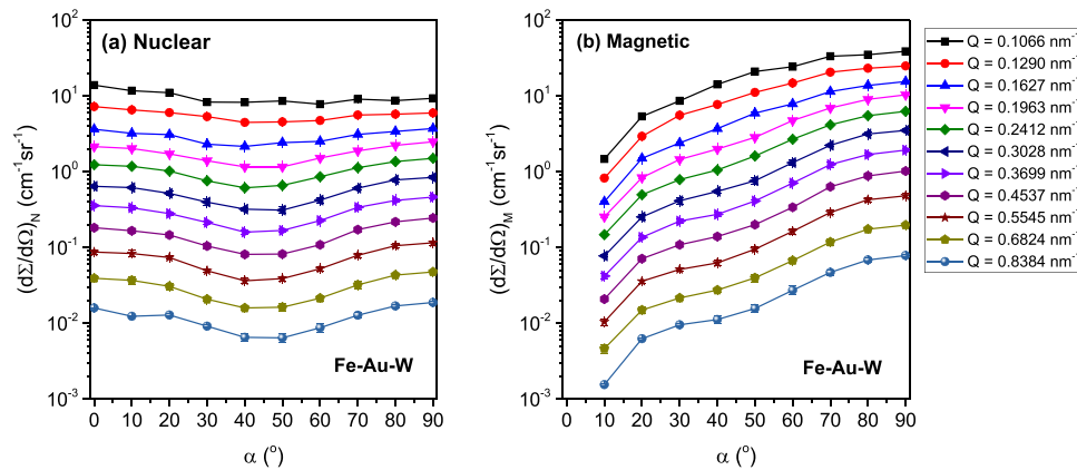
Fig. 8. Angular SANS profiles for the Fe-Au-W alloy measured at room temperature after 12 h of aging at 650 °C showing the scattered intensity (d\Sigma/d\Omega)(Q) as a function of the azimuth angle \alpha with respect to the applied field at \alpha = 0^\circ . The SANS patterns are shown for different values for the wave vector transfer Q . The panels indicate: (a) nuclear scattering (d\Sigma/d\Omega)_N(Q) and (b) magnetic scattering \sin^2(\alpha)(d\Sigma/d\Omega)_M(Q) .
