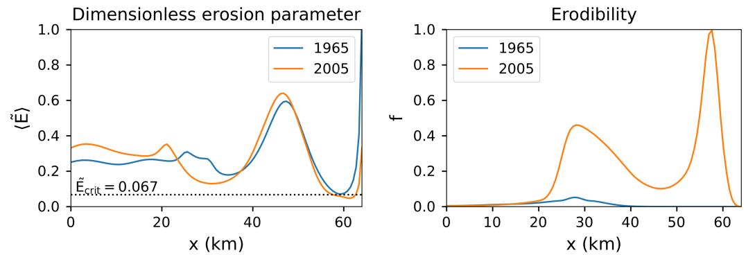
Figure 9. Dimensionless erosion parameter \tilde{E} and erodibility f for 1965 and 2005 with average summer discharge ( Q = 40 \text{ m}^3/\text{s} ). (left) The dimensionless erosion parameter (See equation (14)) and its threshold value 0.067. If \langle \tilde{E} \rangle exceeds the threshold, local resuspension does not restrict the maximum suspended sediment concentration. (right) The erodibility f , which is a measure for the availability of easily erodible sediment. A value f < 1 indicates that sediment availability is limiting the sediment concentration, while f = 1 indicates that local resuspension is limiting the sediment concentration.
