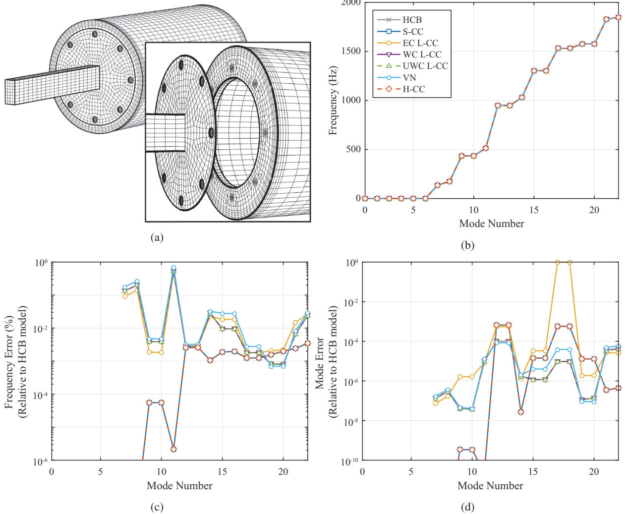
Figure 10: FE mesh (a), natural-frequency comparison (b), frequency-error comparison (c), and mode-error comparison (d) for the can-beam model.
