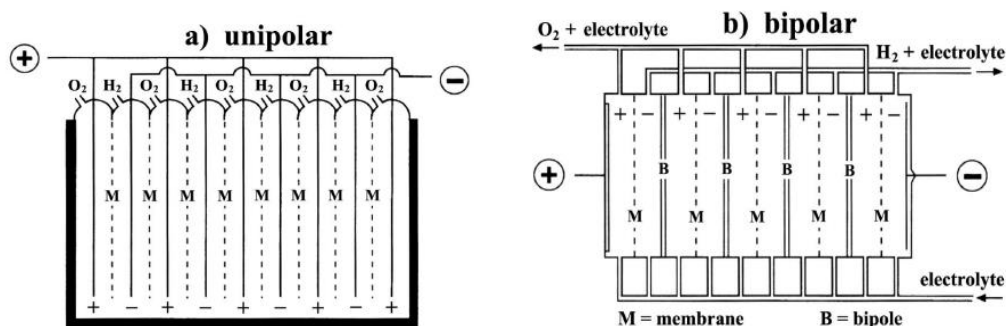
Figure 52. Electrolysis units with (a) unipolar and (b) bipolar cell configurations (Santos, 2013)
