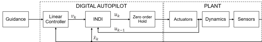
Fig. 3 INDI autopilot architecture
