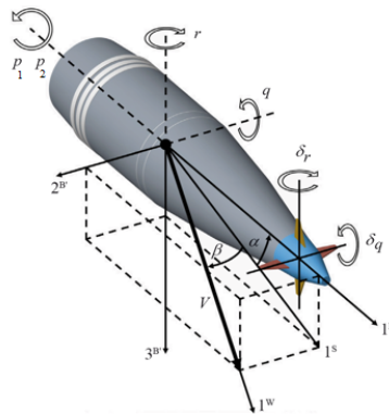
Fig. 1 Decoupled Fuze Guided Projectile
