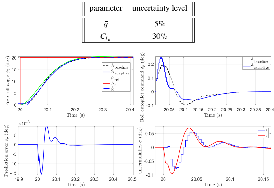
Fig. 14 Performance comparison between the roll baseline autopilot and the \mathcal{L}_1 adaptive augmentation
