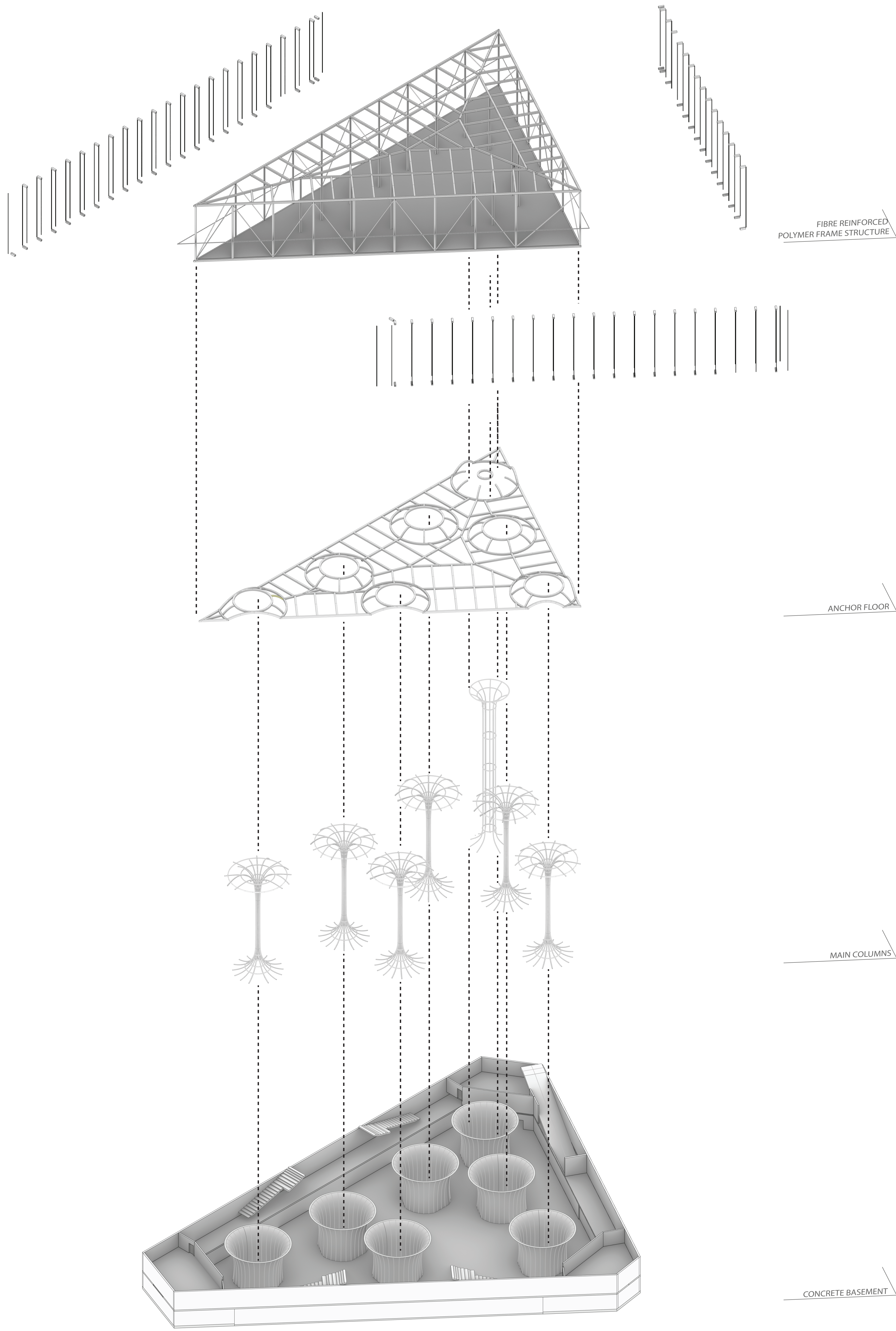
Exploded View Structure
