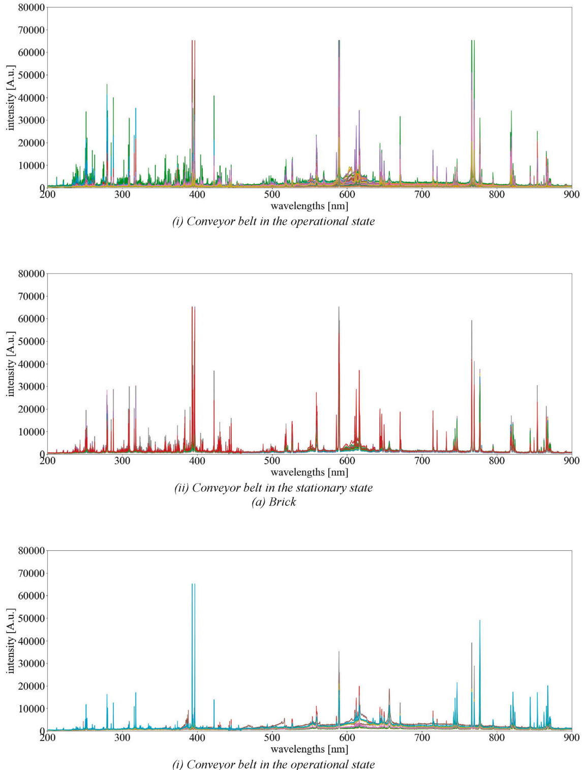
Fig. 11. Comparison of spectra of different materials in the operation and stationary states of the conveyor belt.
