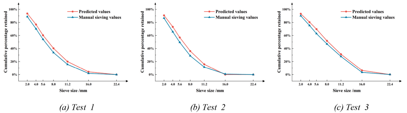
Fig. 8. Cumulative percentage retained graphs.
