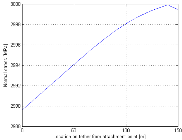
Figure 13.5: Tether normal stress (no safety factor and V = V_{\text{extreme}} )
