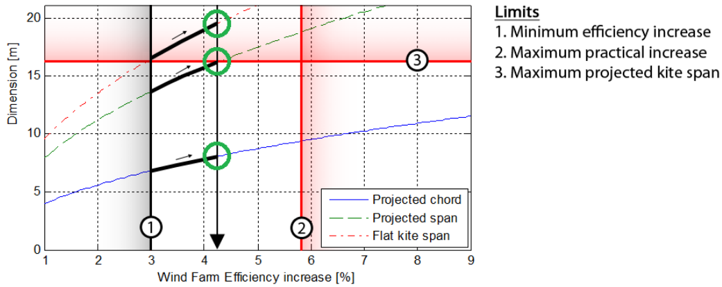
Figure 11.4: Final design space, with final kite dimensions and efficiency increase
