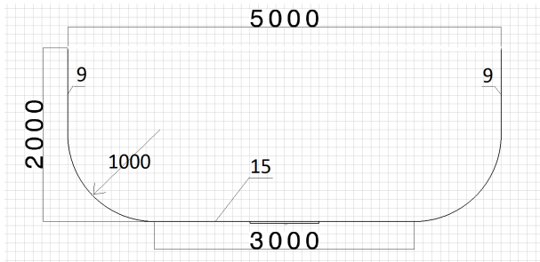
Figure 14.7: Basic dimensions of the lower structure of the buoy
