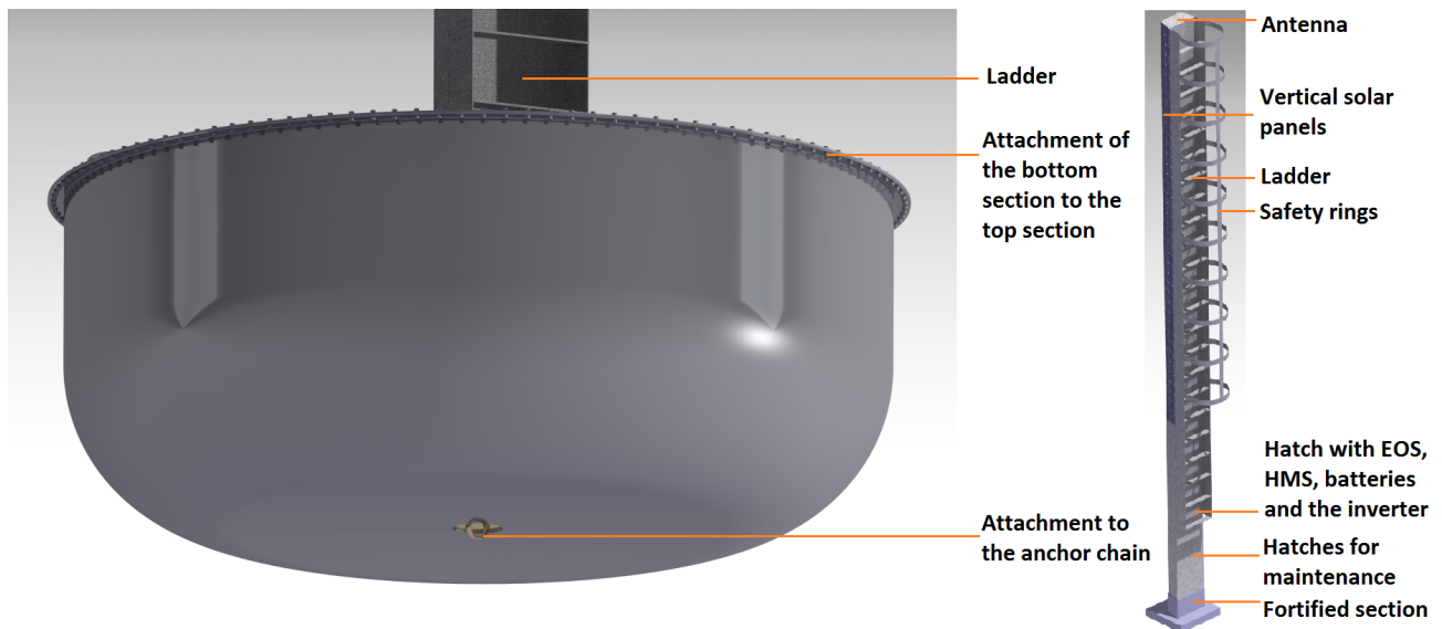
Figure 19.7: The shape of the buoy body, to the left and the mast, to the right
