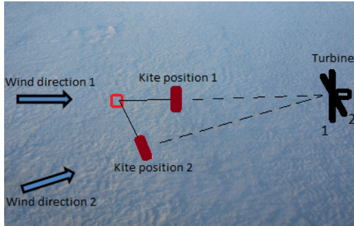
Figure 5.5: The optimal kite position for two different wind directions
