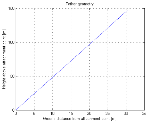
Figure 13.3: The tether geometry ( V = V_{\text{extreme}} )
