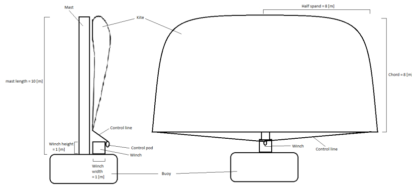
Figure 18.7: Determination of the suspended control line height
