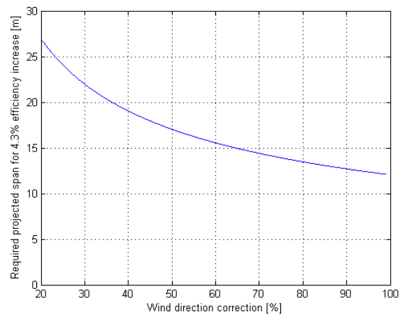
Figure 23.4: Relation between the wind direction correction and the projected kite span.
