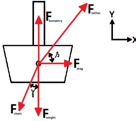
Figure 14.12: Free body diagram of the buoy
