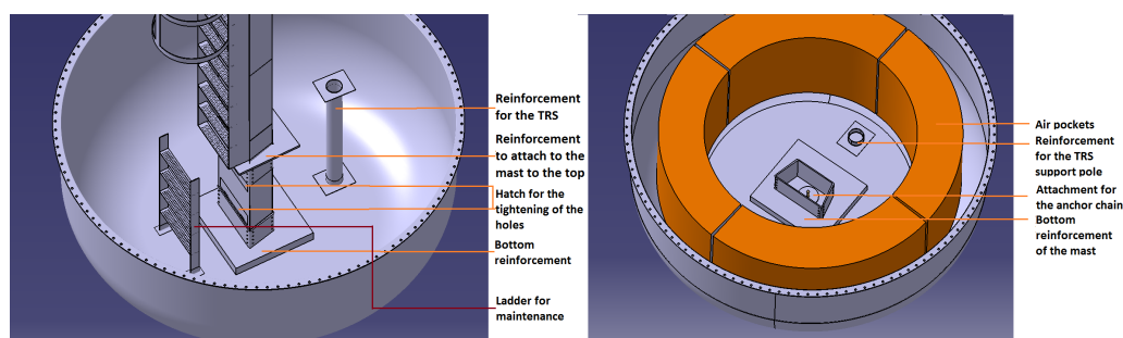
Figure 19.8: The anchoring of the mast to the buoy body, to the left and the air pockets in the buoy, to the right
