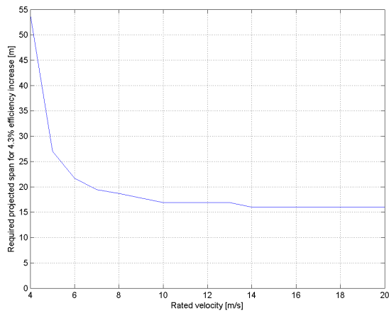
Figure 23.1: Relation between the rated velocity and the projected kite span.
