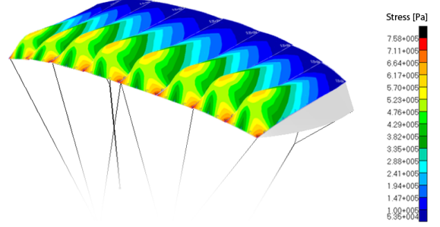
Figure 13.13: Impression of the deformation of and stresses in the kite with 8 sections
