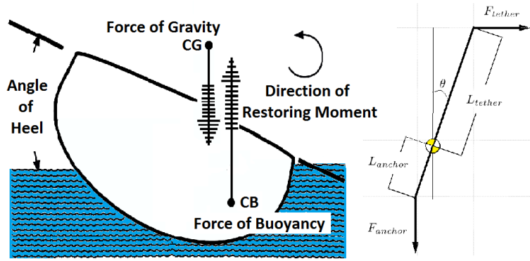
Figure 12.9: Visualisation of the displacement of the centre of buoyancy, and associated metacentre
