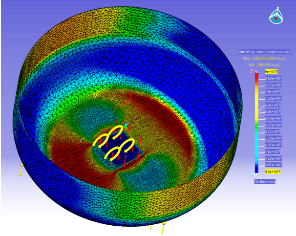
Figure 14.9: Top view of the modelled forces and resulting Von Mises stresses
