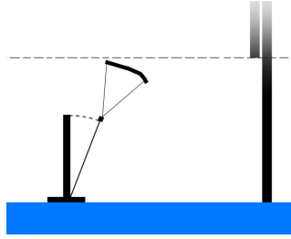
Figure 11.1: Schematic of the structural limit imposed by the tether and bridle system length
