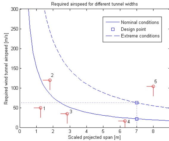
Figure 26.1: The relation between the (scaled) projected span and the required tunnel airspeed
