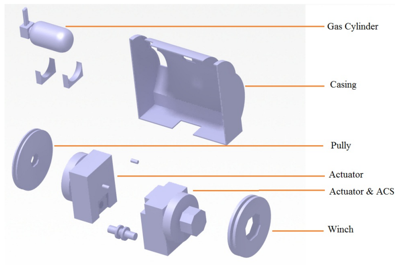
Figure 18.8: CATIA Exploded View of Control Pod
