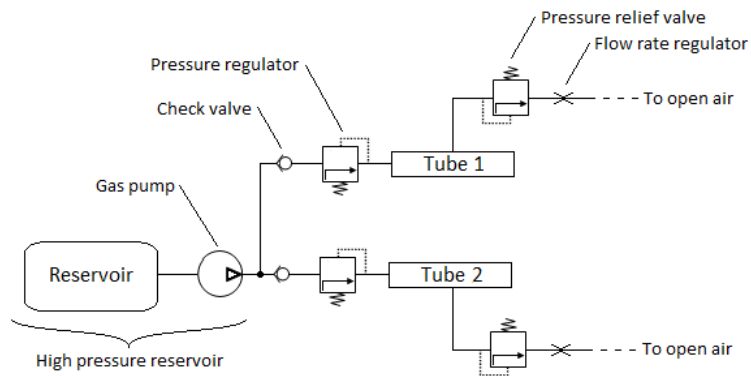
Figure 5.4: The pressure regulation system
