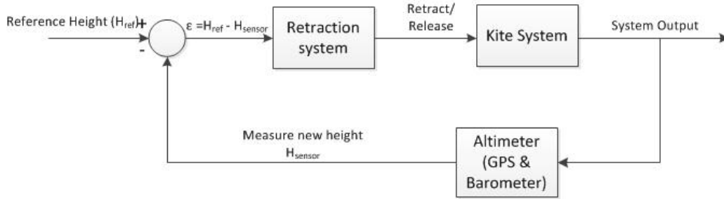
Figure 12.8: Control flow Retraction
