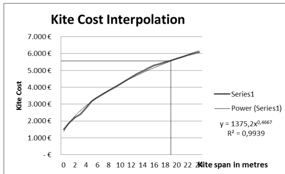
Figure 22.2: Kite Cost Function
