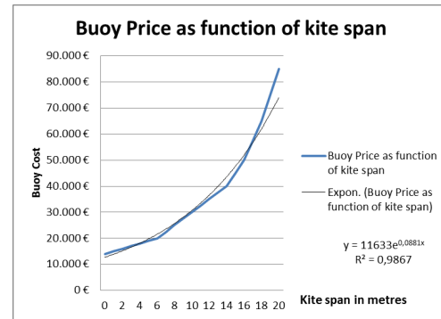
Figure 22.3: Buoy Cost Function
