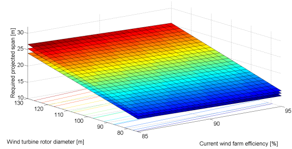
Figure 23.6: 4D-multi applicability plot for a wind direction correction factor of 0.57
