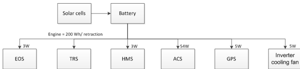
Figure 6.4: Electric Block Diagram
