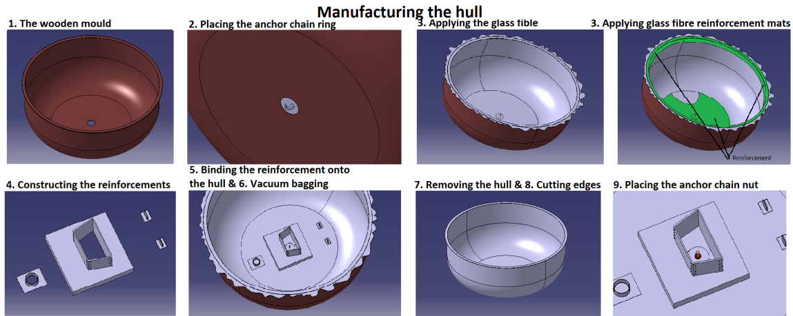
Figure 16.2: Manufacturing the hull in steps
