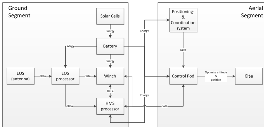
Figure 6.2: Hardware Block Diagram
