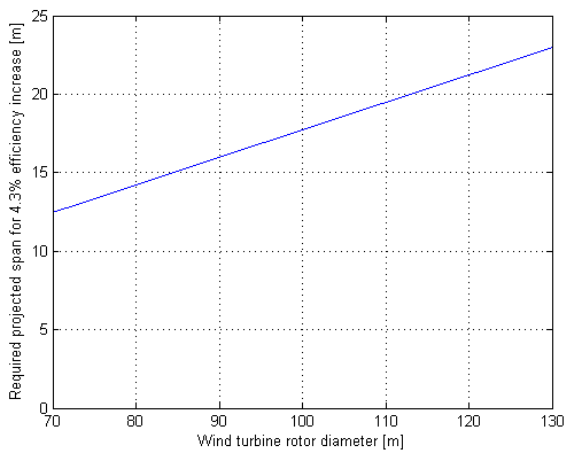
Figure 23.3: Relation between the rotor diameter and the projected kite span.
