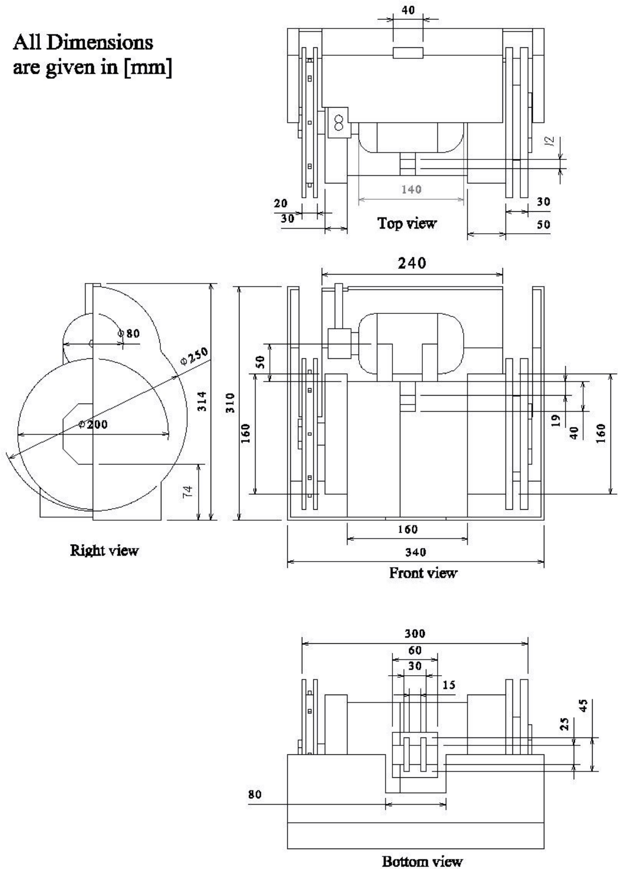
Figure 18.9: CATIA Detailed Sketch of Control Pod
