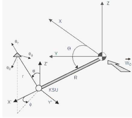
Figure 12.2: Kite Reference System
