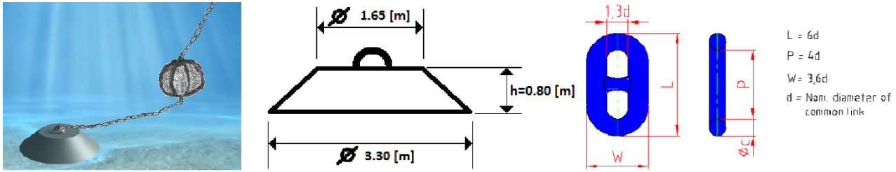
Figure 14.13: Underwater segment, layout and dimensions
