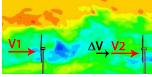
Figure 10.1: Sketch of the small wind farm with velocity definitions
