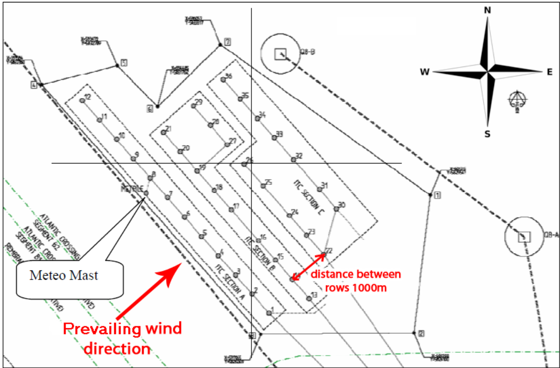
Figure 1.2: Layout of the OWEZ wind farm [2]
