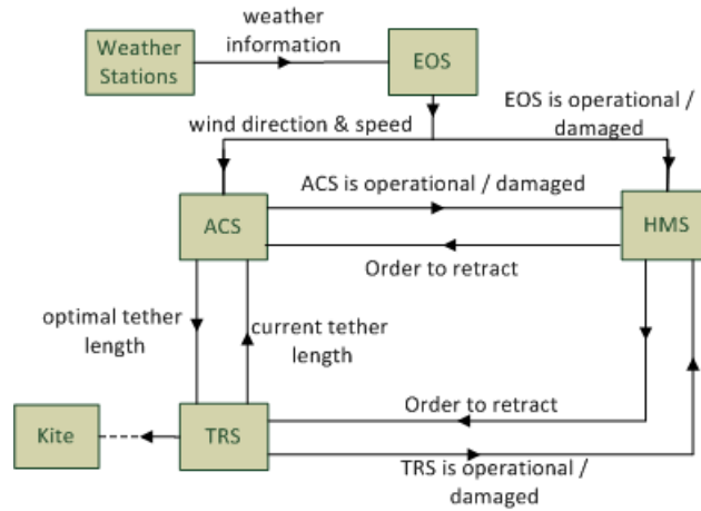
Figure 6.1: Data Handling Block Diagram
