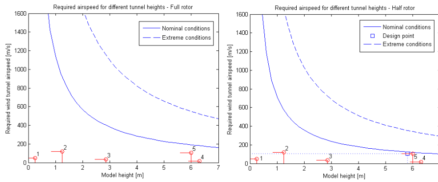
Figure 26.4: The relation between the (scaled) model height and the required tunnel airspeed
