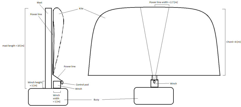
Figure 18.5: Determination of the power line length
