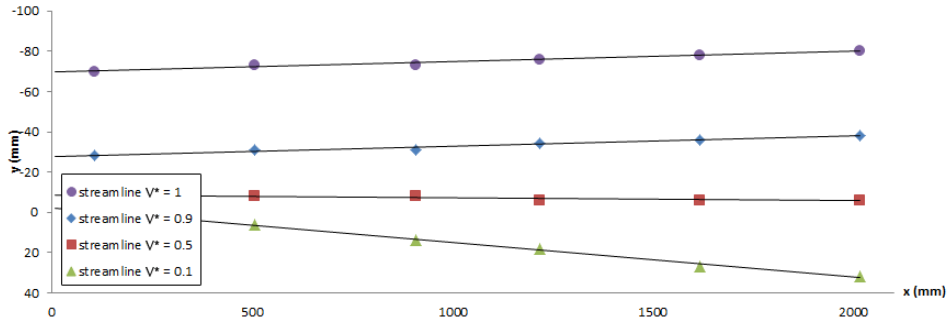
Figure 10.10: Streamlines in the wind tunnel transformed in y-coordinates in [mm] (derived from wind tunnel test [22])
