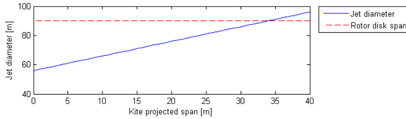
Figure 10.13: Diameter of the jet left by the kite at location of the wind turbine downstream
