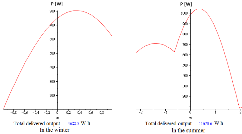
Figure 19.5: Total power output of a combination of vertically and horizontally placed solar panels during winter
