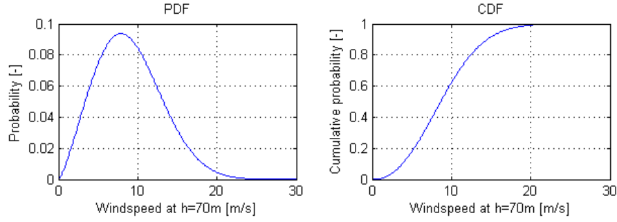
Figure 10.2: Distribution of the average windspeed on 70 [m].
