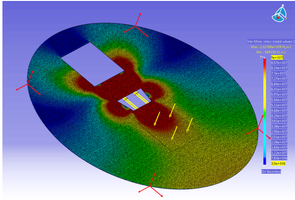
Figure 14.5: Von Mises stress distribution over the top panel of the buoy
