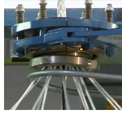
Figure 16.1: The manufacturing of a tether with an electricity cable inside it
