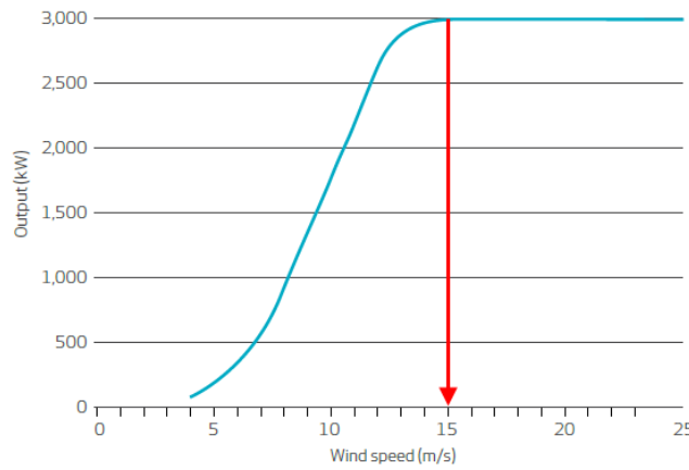
Figure 10.5: Power curve of the Vestas V90-3MW (figure from [14])
