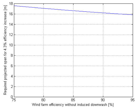
Figure 23.2: Relation between the current wind farm efficiency and the projected kite span.
