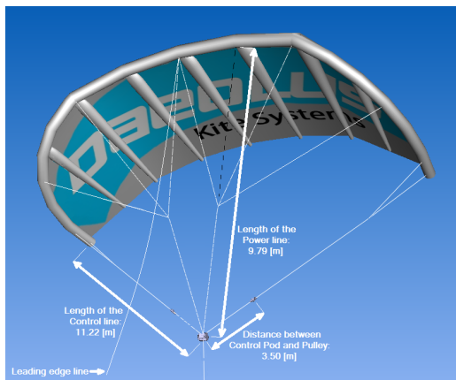
Figure 18.1: Three-dimensional view of kite
