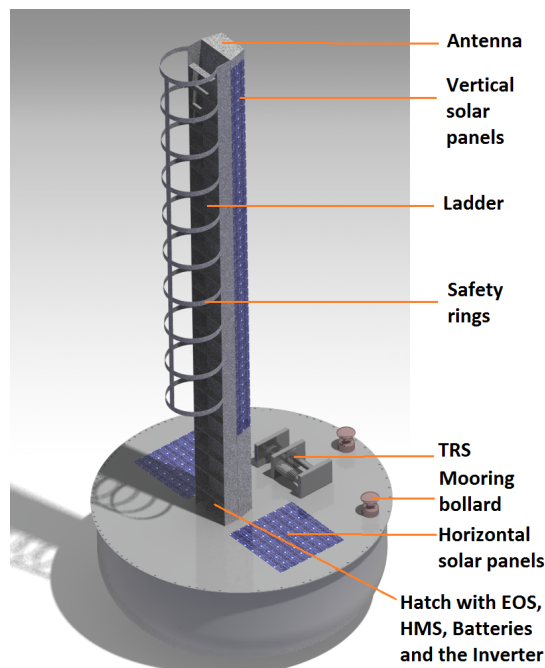
Figure 19.1: The overview of the ground segment
