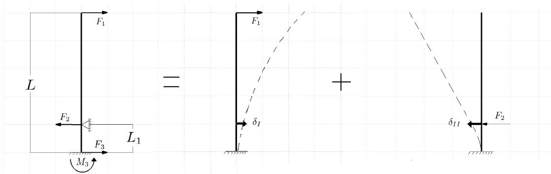
Figure 14.1: FBD's and equivalent virtual structures
