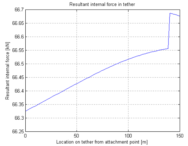
Figure 13.4: The tether force ( V = V_{\text{extreme}} )
