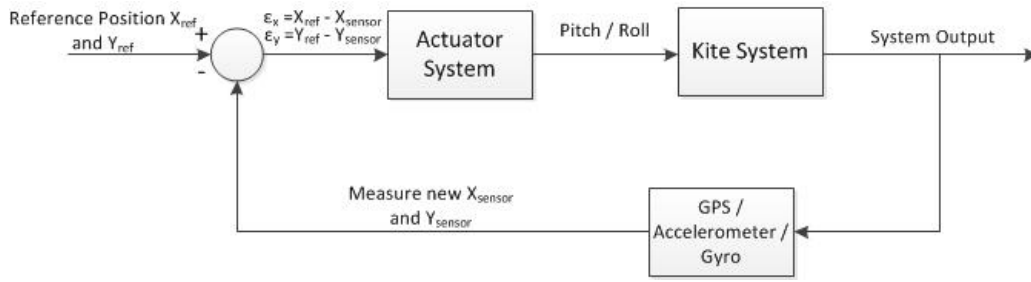
Figure 12.7: Control Flow Actuator
