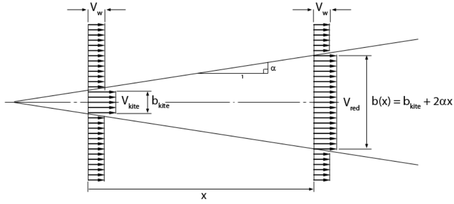
Figure 10.12: Linear jet model (based on the Jensen wake model [20][17])
