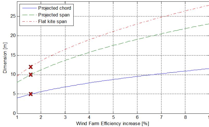
Figure 10.18: Relationship between kite dimensions and wind farm efficiency increase (the X's mark the results of the example calculation)
