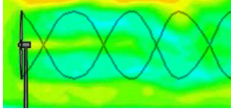
Figure 10.9: Vortices induced by the wind turbine blades forming helices behind the wind turbine.
