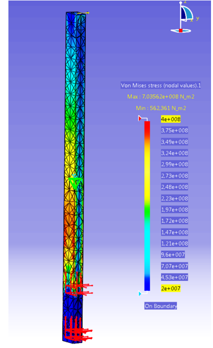
Figure 14.4: Von Mises stresses
