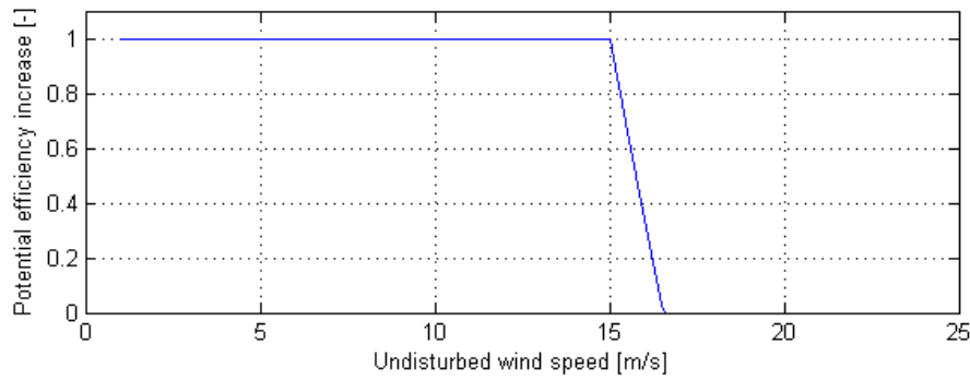
Figure 10.7: Potential efficiency increase (on a scale from 0 to 1) for each wind speed
