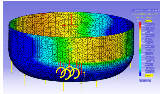
Figure 14.8: Side view of the modelled forces and resulting Von Mises stresses
