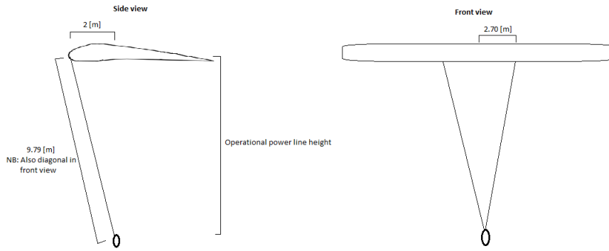
Figure 18.6: Determination of the operational power line height
