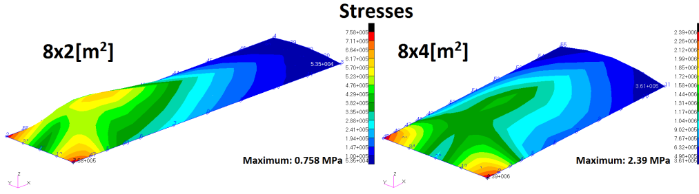
Figure 13.10: Internal stresses in the skin for a 8x2 [m 2 ] and a 8x4 [m 2 ] kite element.
