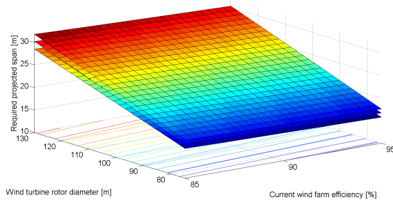
Figure 23.5: 4D-multi applicability plot for a wind direction correction factor of 0.40
