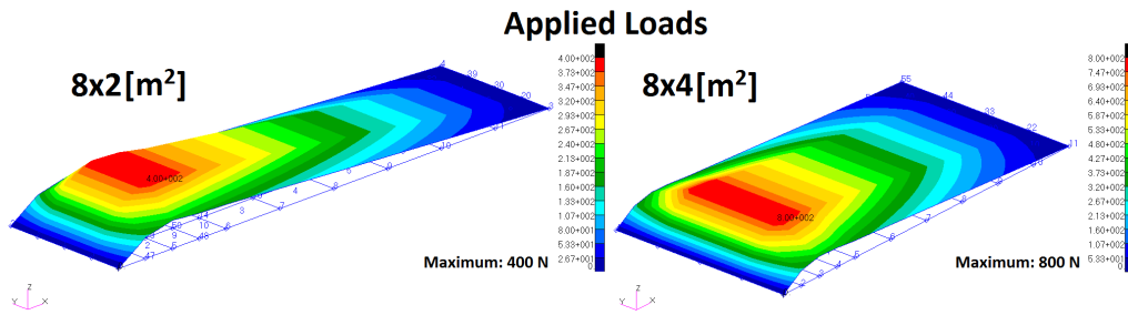
Figure 13.8: The applied loads on the skin for a 8 \times 2 [m 2 ] and a 8 \times 4 [m 2 ] kite element.
