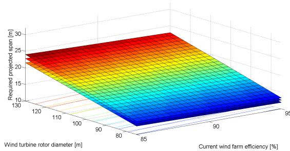
Figure 23.7: 4D-multi applicability plot for a wind direction correction factor of 0.70
