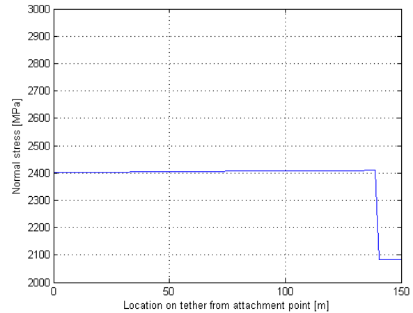
Figure 13.6: Tether normal stress (with safety factor and V = V_{\text{extreme}} )
