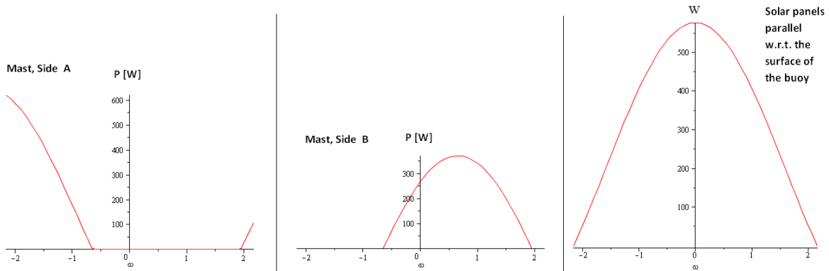
Figure 19.4: Power output of the horizontal and vertical placed solar cells during summer conditions
