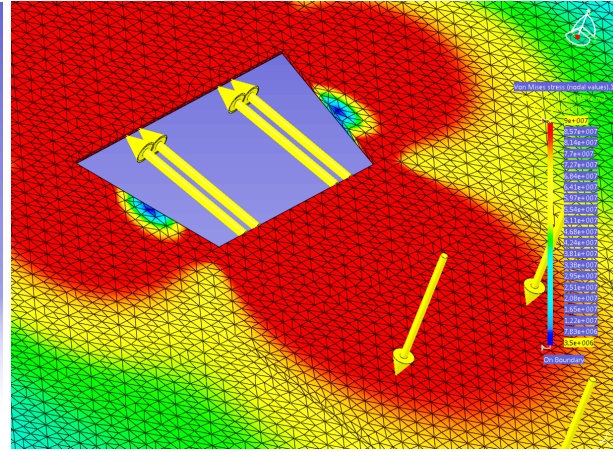
Figure 14.6: Von Mises stress distribution near the hole for the mast
