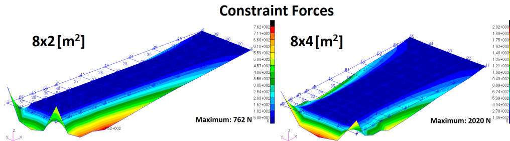
Figure 13.9: The constraint forces acting on the surrounding inflatable tubes for a 8 \times 2 [m 2 ] and a 8 \times 4 [m 2 ] kite element.
