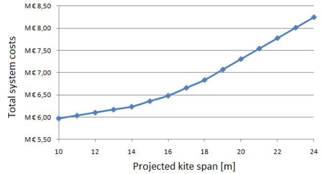
Figure 23.8: Total system costs vs. the projected kite span
