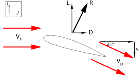
Figure 10.15: Lift by bending the flow
