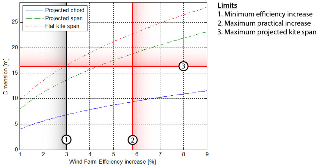
Figure 11.3: Final design space
