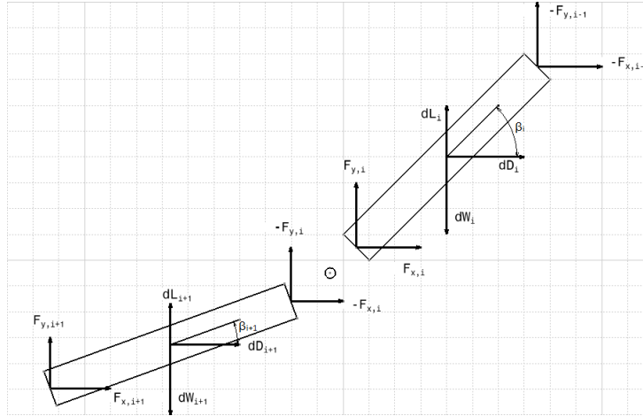
Figure 13.2: Two rigid beam elements and the forces acting on them
