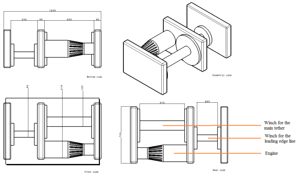
Figure 19.6: The overview of the TRS
