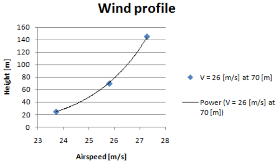
Figure 11.8: Wind profile calculation for V_{wind} = 26 [m/s] at hub height
