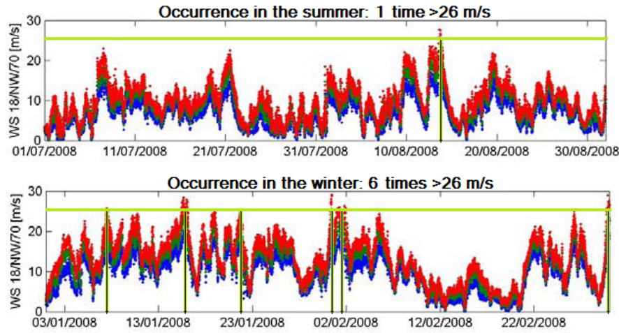
Figure 11.7: Frequency of occurrence of V_{wind} > 26 [m/s] at the height of the hub
