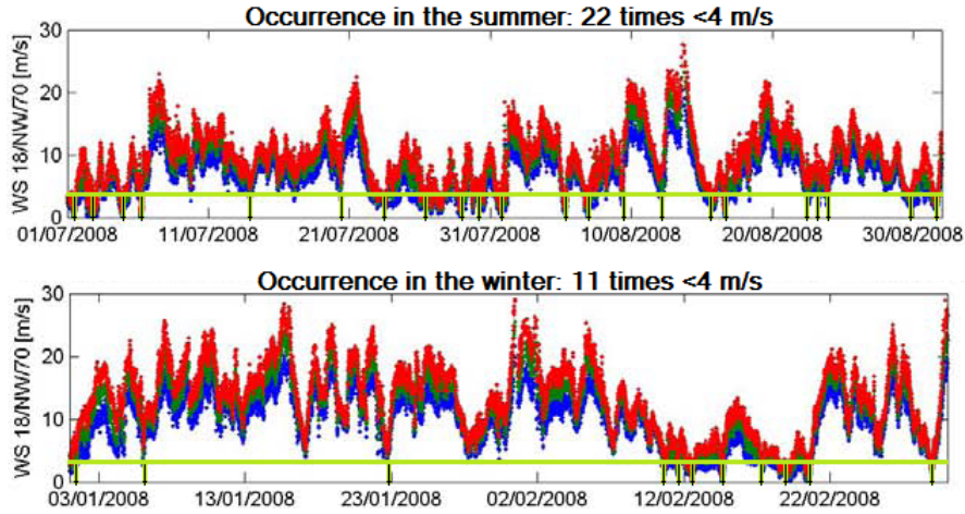
Figure 11.6: Frequency of occurrence of V_{wind} < 4 \text{ [m/s]}
