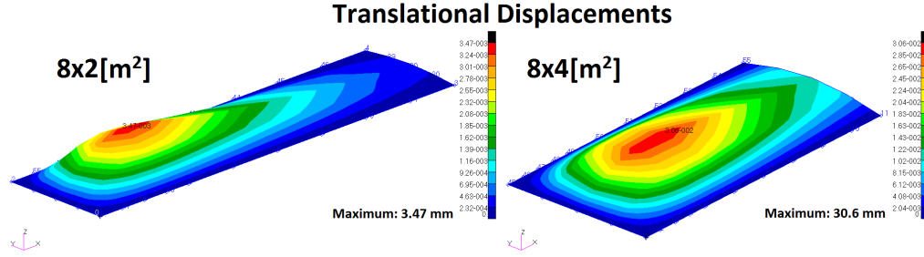
Figure 13.11: Translational displacements of the skin for a 8x2 [m 2 ] and a 8x4 [m 2 ] kite element.
