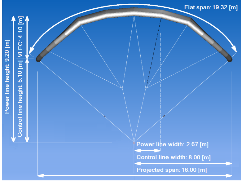
Figure 18.4: Front view of the kite
