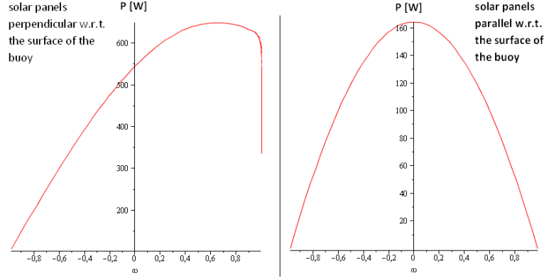
Figure 19.3: Power output of the horizontal and vertical placed solar cells during winter conditions
