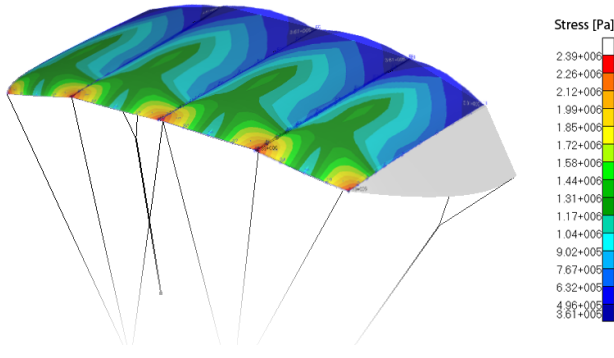
Figure 13.12: Impression of the deformation of and stresses in the kite with 4 sections
