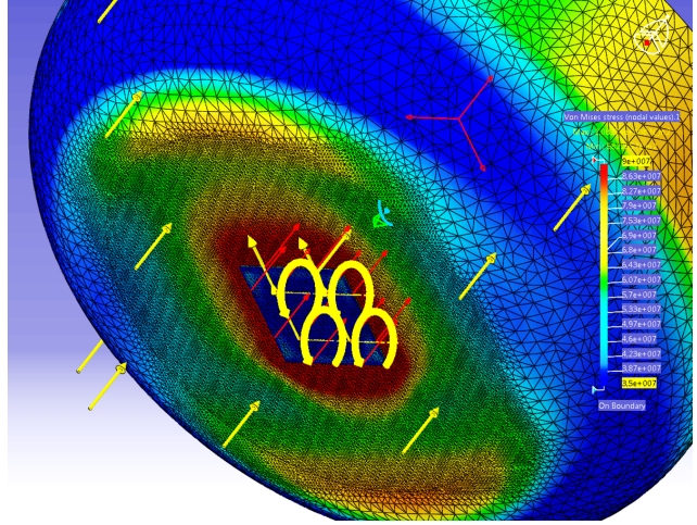
Figure 14.10: Bottom view of the modelled forces and resulting Von Mises stresses
