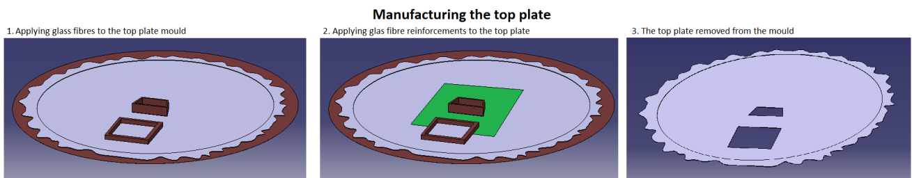
Figure 16.3: Manufacturing the top plate in steps
