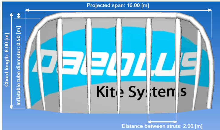
Figure 18.2: Bottom view of the kite
