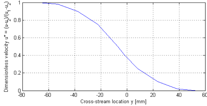
Figure 10.11: Velocity profile of the developed mixing layer (calculated from wind tunnel test data [22])
