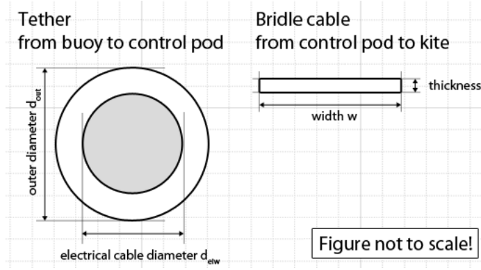
Figure 13.1: Different cross sections of different parts of the tether
