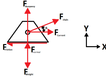
Figure 14.11: Free body diagram of the anchor
