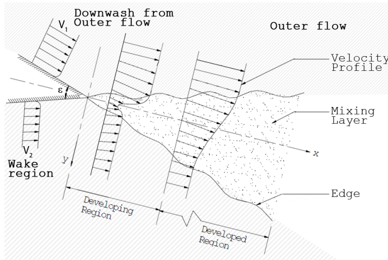
Figure 10.8: Sketch of the mixing layer (figure based on [22])
