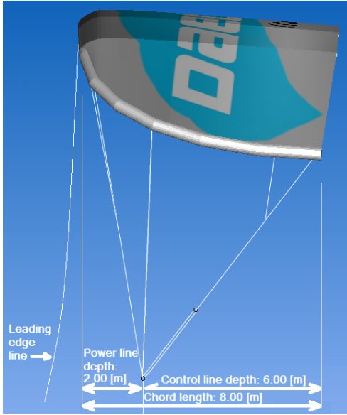
Figure 18.3: Right view of the kite
