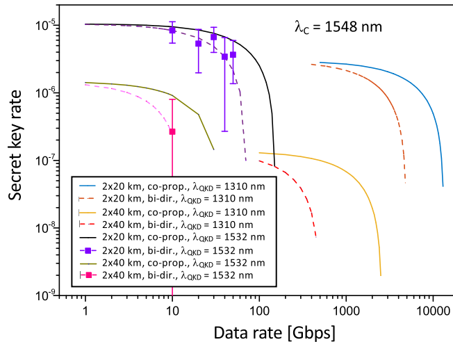
Figure 3. Results. Predicted (lines) and experimentally obtained (squared) secret key rates (per clock cycle and assuming the infinite key limit) for different fiber lengths, data rates, wavelengths of the quantum channel, and assuming bi-directional or uni-directional (co-propagating) classical communication between Alice and Bob (connected via Charlie). Classical data is assumed to be at \lambda_C = 1548 nm wavelength. Experimental error bars indicate one standard deviation and are obtained assuming Poisson detection statistics.
