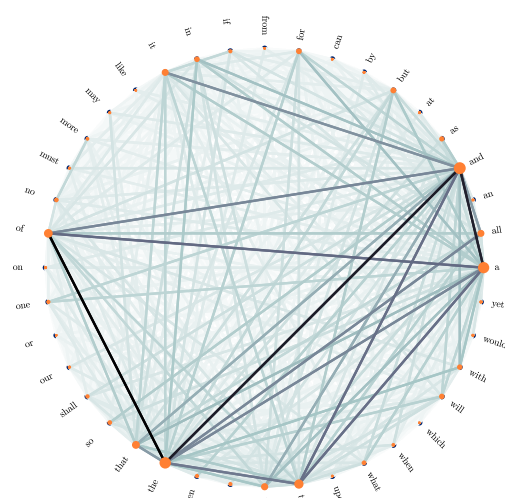
Fig. 2. Example of word adjacency network for the author Robert Louis Stevenson.
