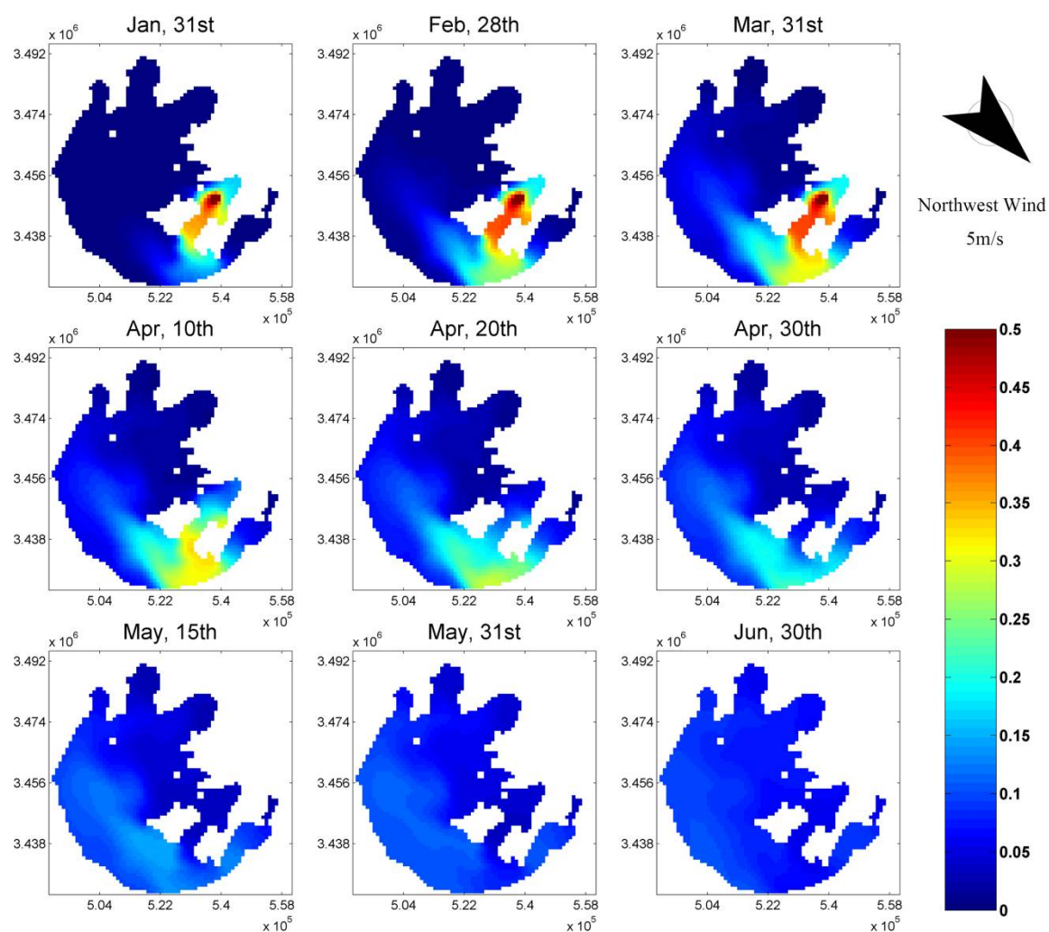
Figure 16. Time series of tracer concentration images, with the model driven by constant 5 m/s northwest wind. Unit in the figure is kg/m 3 .
