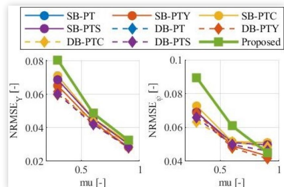
FIGURE 14 Tracking KPIs variation due to friction coefficient.
