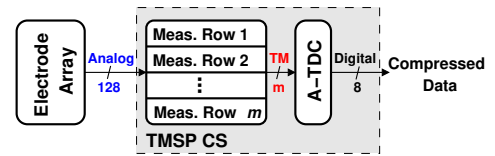
Figure 1. Proposed TMSP CS system high-level block diagram.
