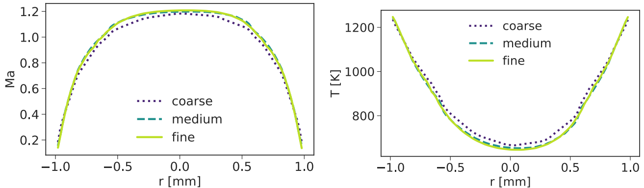
Fig. 13. Mach number and temperature profile at the outlet of the second nozzle for different grids (see Table 7).
