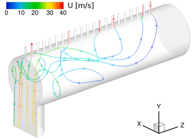
Fig. 4. Streamlines colored by velocity magnitude, where values above 40 \text{ms}^{-1} are clipped. (For interpretation of the references to color in this figure legend, the reader is referred to the web version of this article.)
