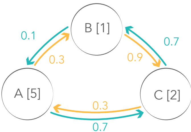
Figure 8 - Example state model with three values
