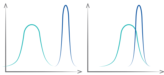
Figure 6 - Overlapping mixture models, hard vs. soft clustering
