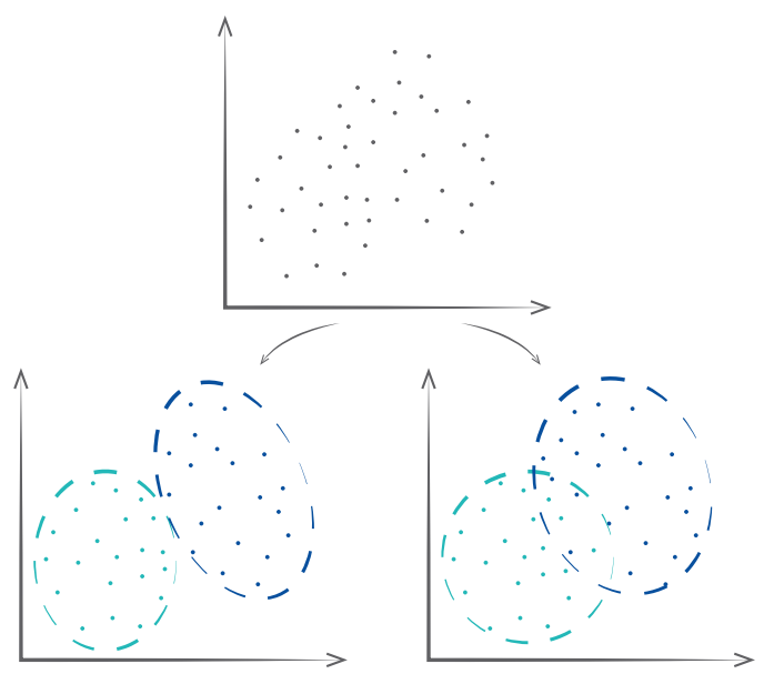
Figure 5 - Difference soft/hard clustering
