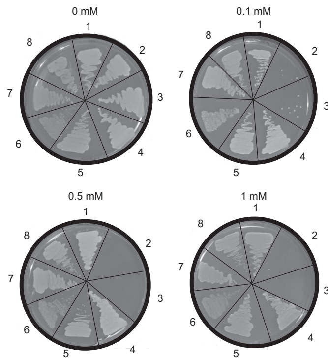
Fig. 2. Growth inhibition by L-tyrosine of the reference S. cerevisiae strain CEN.PK113-7D and strains engineered in key steps of aromatic amino acid biosynthesis. The yeast strains were streak on SM medium with 2% glucose containing either 0 (left top panel), 0.1 mM (right top panel), 0.5 mM (left bottom panel) or 1 mM (right bottom panel) L-tyrosine. Plates were incubated at 30 °C for 52 h. 1: CEN.PK113-7D (prototrophic reference strain) 2: CEN.PK532-1A ( aro3Δ ARO4 ) 3: CEN.PK666-1C ( aro3Δ TP1p-ARO4 ) 4: CEN.PK718-5A ( aro3Δ ARO4 K229L ) 5: IMZ014 ( aro3Δ ARO4 K229L TDH3-ARO7 ) 6: IMZ018 ( aro3Δ ARO4 K229L TDH3-ARO7 G141S ) 7: IMZ016 ( TDH3-ARO7 ) 8: IMZ017 ( TDH3-ARO7 G141S ).
