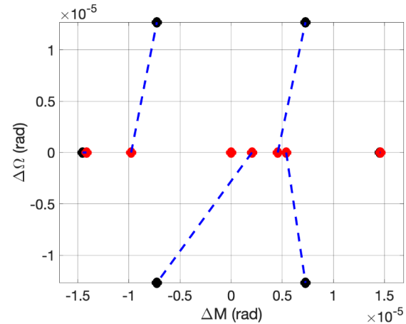
Fig. 1. Formation distribution from the along-track direction (in red) to the hexagonal formation (in black). The final and initial position in the \Delta M - \Delta \Omega plane of each spacecraft is connected by a blue dashed line.
