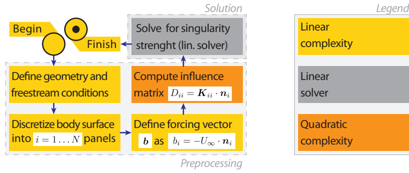
Figure 10. Structure of a conventional panel method
