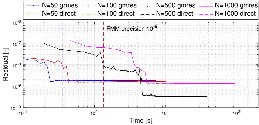
Figure 12. Calculation time for the FastBEM algorithm w.r.t. direct evaluation
