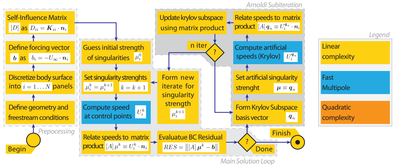
Figure 17. Structure of a stationary FastBEM panel method
