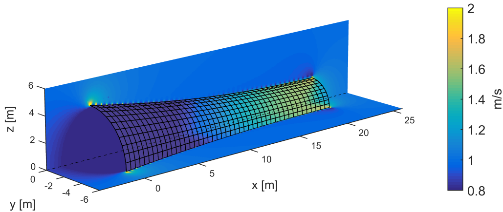
Figure 13. In plane velocity of the nozzle
