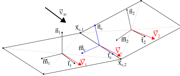
Figure 3. Wake alignment nomenclature
